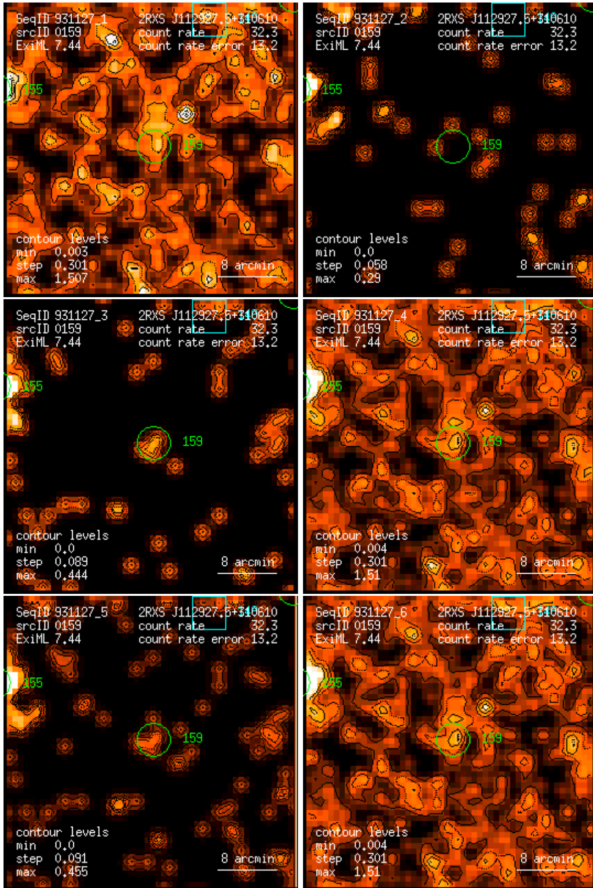
Figure 159: RASS 931127: detection 0159: band rate images, Gaussian filter: (1) PSPC channels 11 – 41, (2) 52 – 90, (3) 91 – 201, (4) 11 – 235, (5) 52 – 201, (6) 11 – 201. Broad band rates in counts/ks. Band rate contour levels in counts/ks/arcmin 2 .
