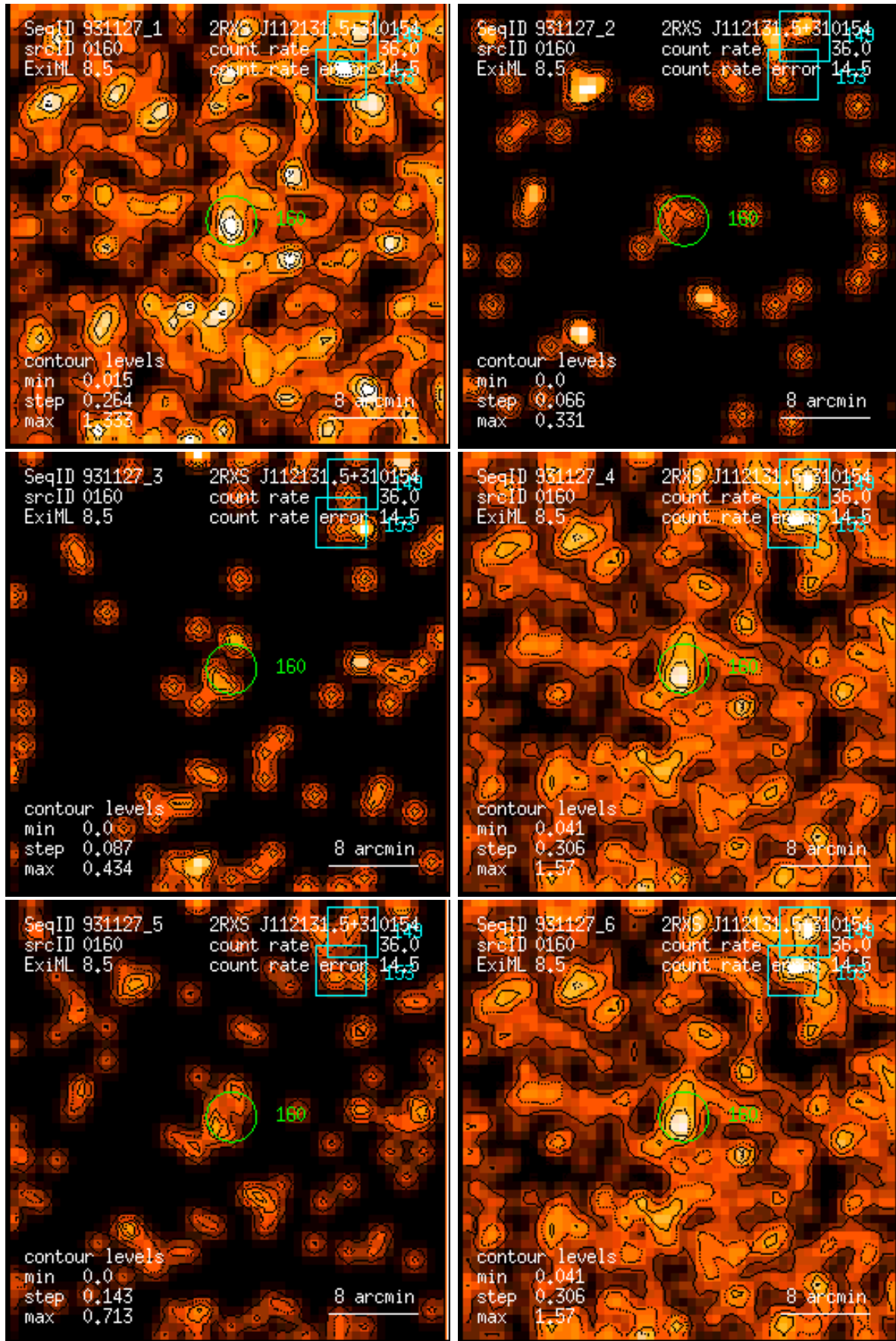
Figure 160: RASS 931127: detection 0160: band rate images, Gaussian filter: (1) PSPC channels 11 – 41, (2) 52 – 90, (3) 91 – 201, (4) 11 – 235, (5) 52 – 201, (6) 11 – 201. Broad band rates in counts/ks. Band rate contour levels in counts/ks/arcmin 2 .
