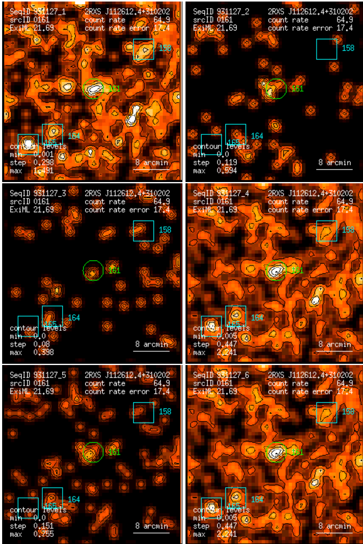
Figure 161: RASS 931127: detection 0161: band rate images, Gaussian filter: (1) PSPC channels 11 – 41, (2) 52 – 90, (3) 91 – 201, (4) 11 – 235, (5) 52 – 201, (6) 11 – 201. Broad band rates in counts/ks. Band rate contour levels in counts/ks/arcmin 2 .
