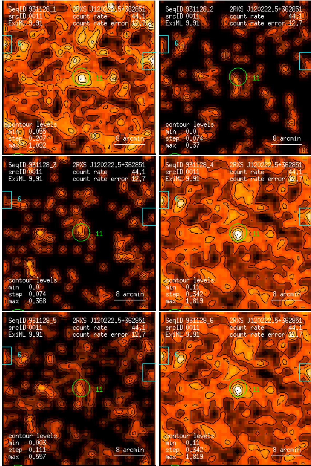
Figure 11: RASS 931128: detection 0011: band rate images, Gaussian filter: (1) PSPC channels 11 – 41, (2) 52 – 90, (3) 91 – 201, (4) 11 – 235, (5) 52 – 201, (6) 11 – 201. Broad band rates in counts/ks. Band rate contour levels in counts/ks/arcmin 2 .
