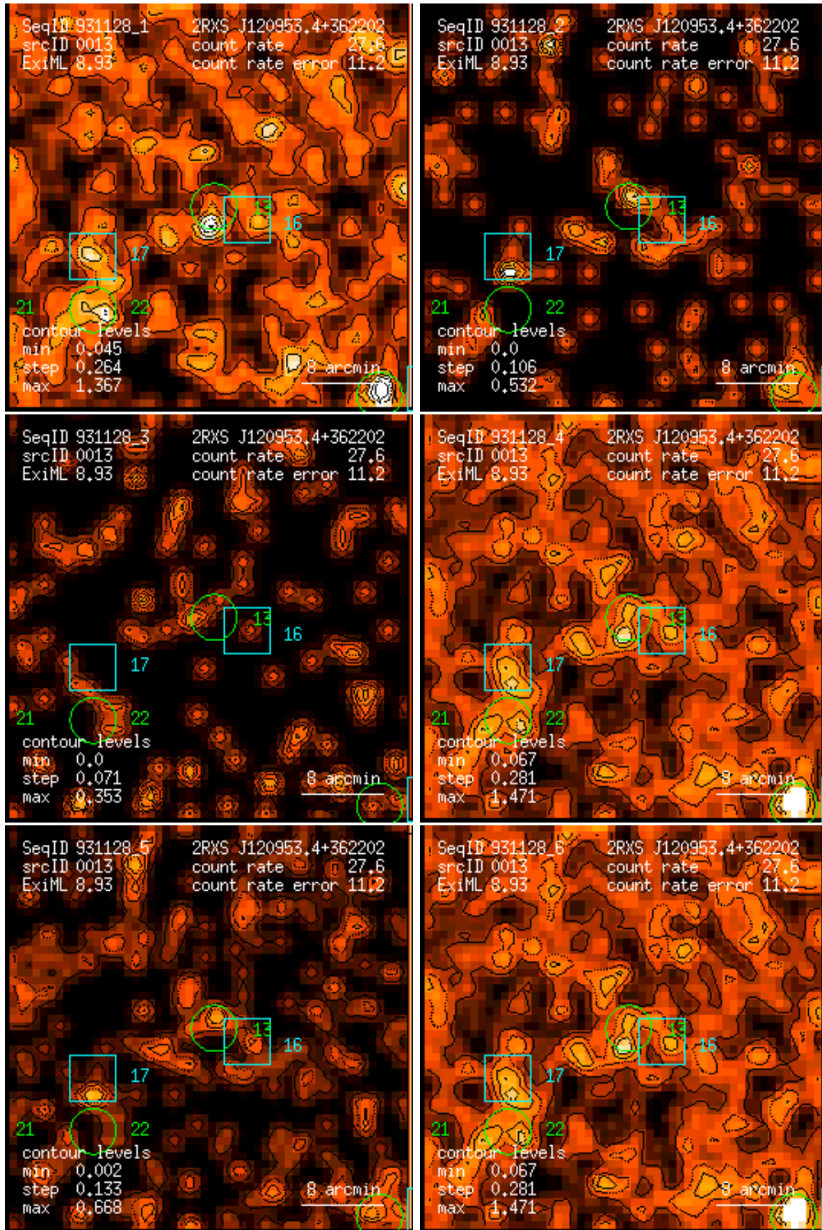
Figure 13: RASS 931128: detection 0013: band rate images, Gaussian filter: (1) PSPC channels 11 – 41, (2) 52 – 90, (3) 91 – 201, (4) 11 – 235, (5) 52 – 201, (6) 11 – 201. Broad band rates in counts/ks. Band rate contour levels in counts/ks/arcmin 2 .
