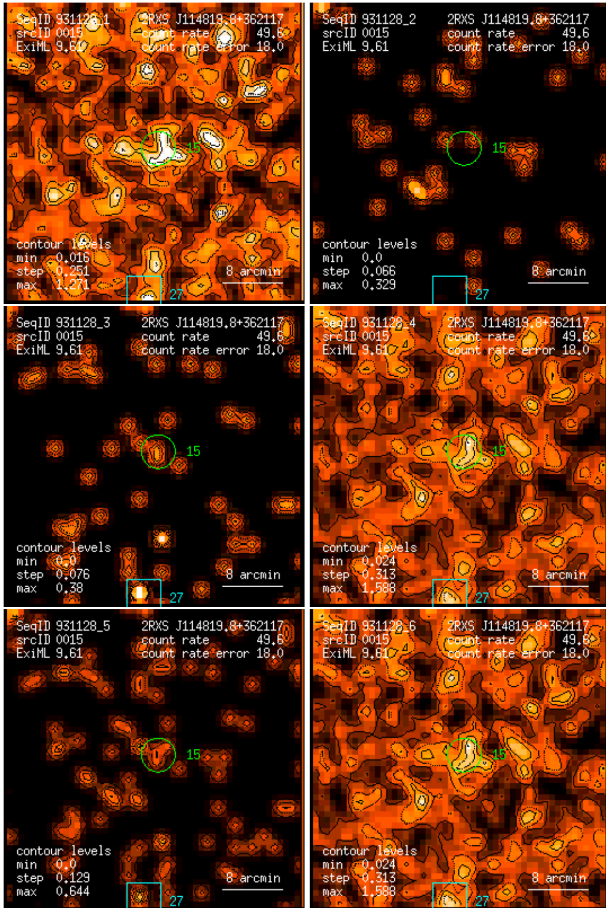
Figure 15: RASS 931128: detection 0015: band rate images, Gaussian filter: (1) PSPC channels 11 – 41, (2) 52 – 90, (3) 91 – 201, (4) 11 – 235, (5) 52 – 201, (6) 11 – 201. Broad band rates in counts/ks. Band rate contour levels in counts/ks/arcmin 2 .
