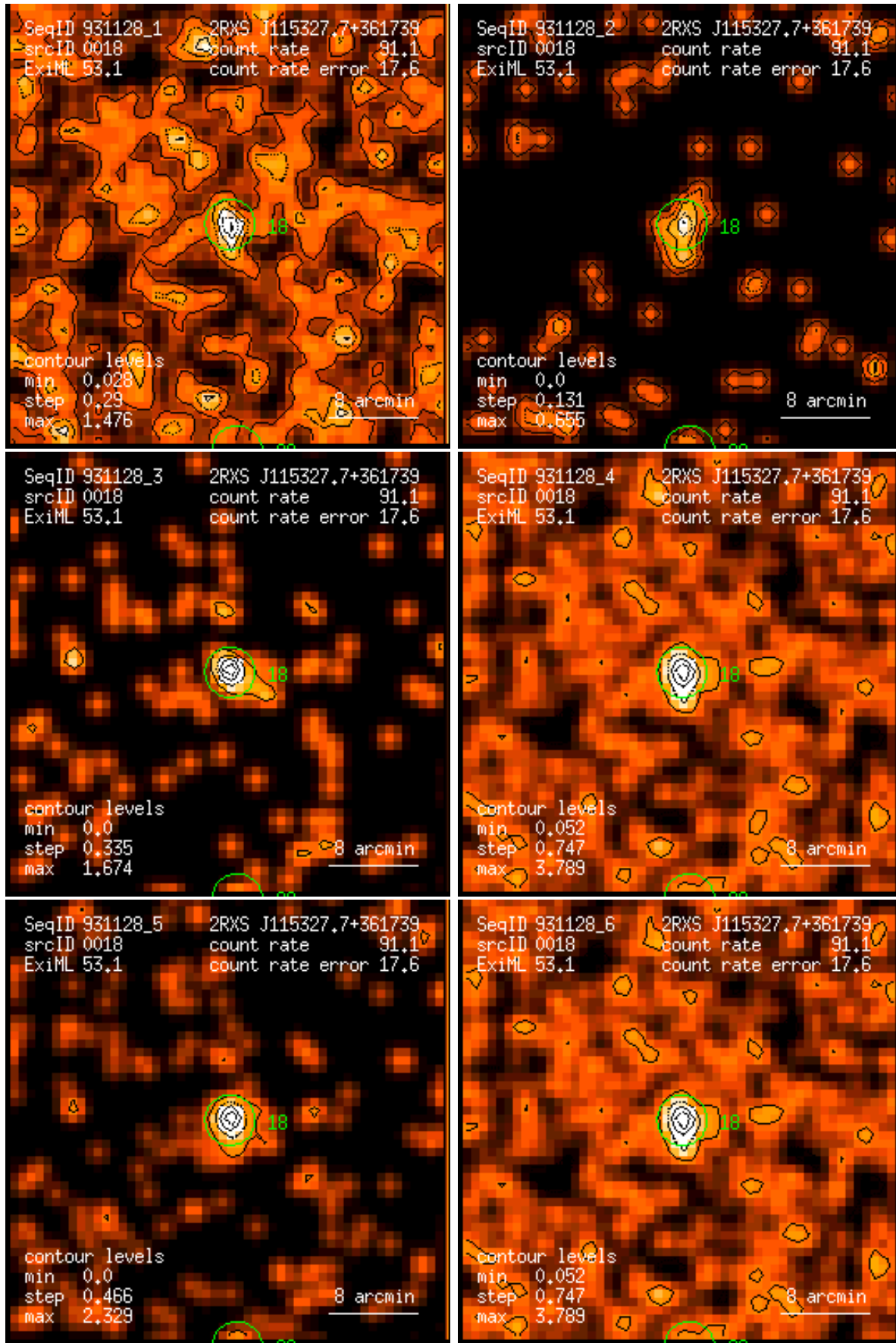
Figure 18: RASS 931128: detection 0018: band rate images, Gaussian filter: (1) PSPC channels 11 – 41, (2) 52 – 90, (3) 91 – 201, (4) 11 – 235, (5) 52 – 201, (6) 11 – 201. Broad band rates in counts/ks. Band rate contour levels in counts/ks/arcmin 2 .
