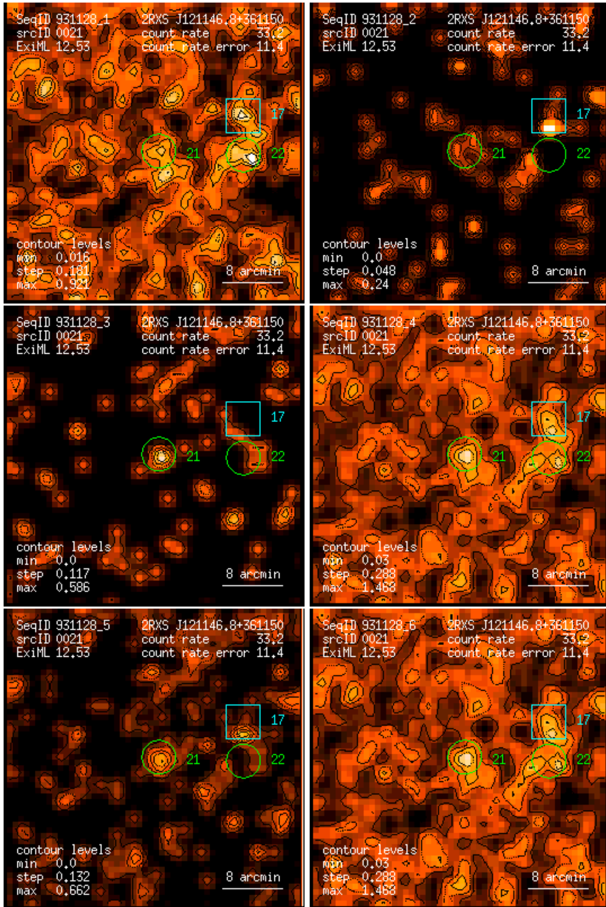
Figure 21: RASS 931128: detection 0021: band rate images, Gaussian filter: (1) PSPC channels 11 – 41, (2) 52 – 90, (3) 91 – 201, (4) 11 – 235, (5) 52 – 201, (6) 11 – 201. Broad band rates in counts/ks. Band rate contour levels in counts/ks/arcmin 2 .
