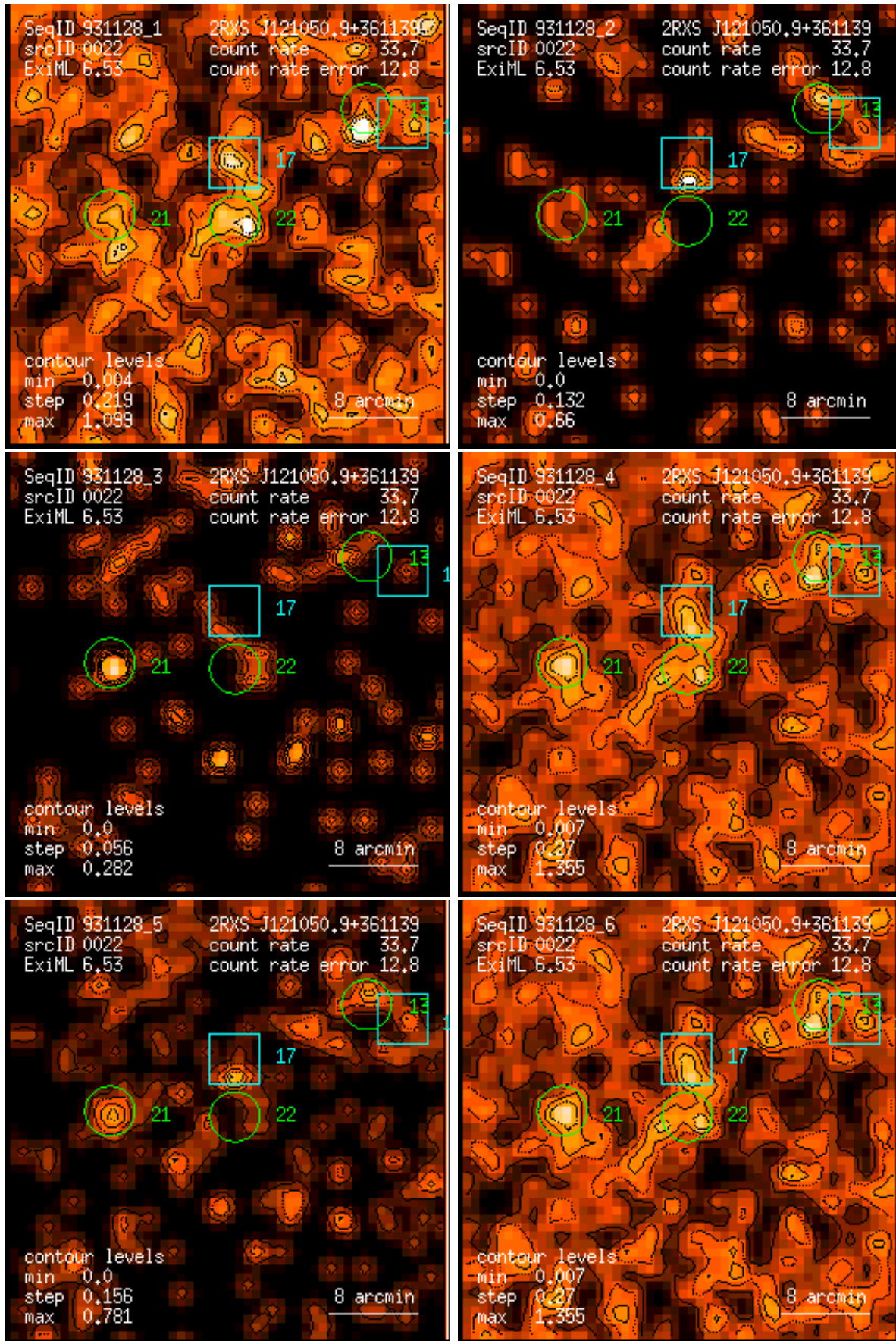
Figure 22: RASS 931128: detection 0022: band rate images, Gaussian filter: (1) PSPC channels 11 – 41, (2) 52 – 90, (3) 91 – 201, (4) 11 – 235, (5) 52 – 201, (6) 11 – 201. Broad band rates in counts/ks. Band rate contour levels in counts/ks/arcmin 2 .
