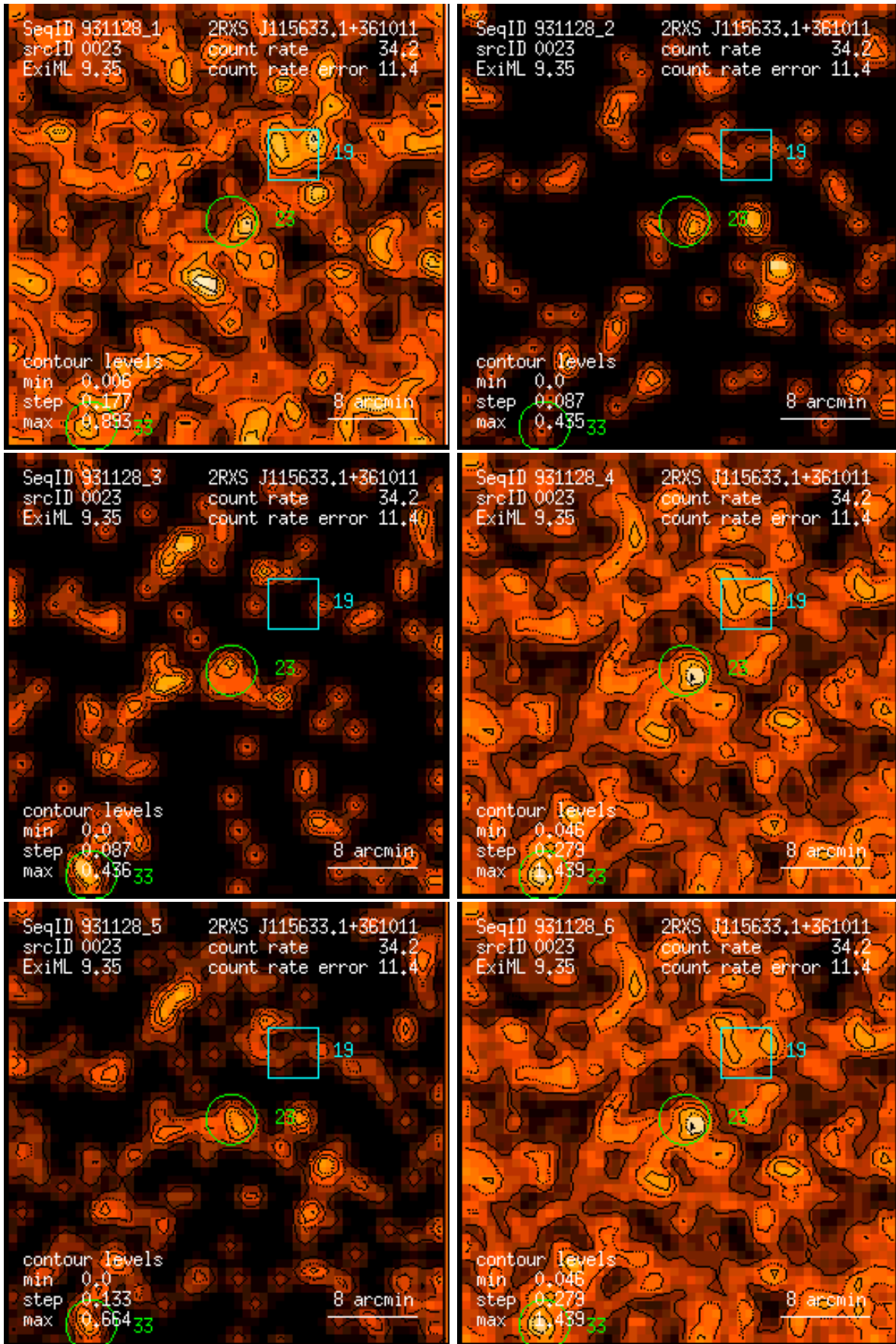
Figure 23: RASS 931128: detection 0023: band rate images, Gaussian filter: (1) PSPC channels 11 – 41, (2) 52 – 90, (3) 91 – 201, (4) 11 – 235, (5) 52 – 201, (6) 11 – 201. Broad band rates in counts/ks. Band rate contour levels in counts/ks/arcmin 2 .
