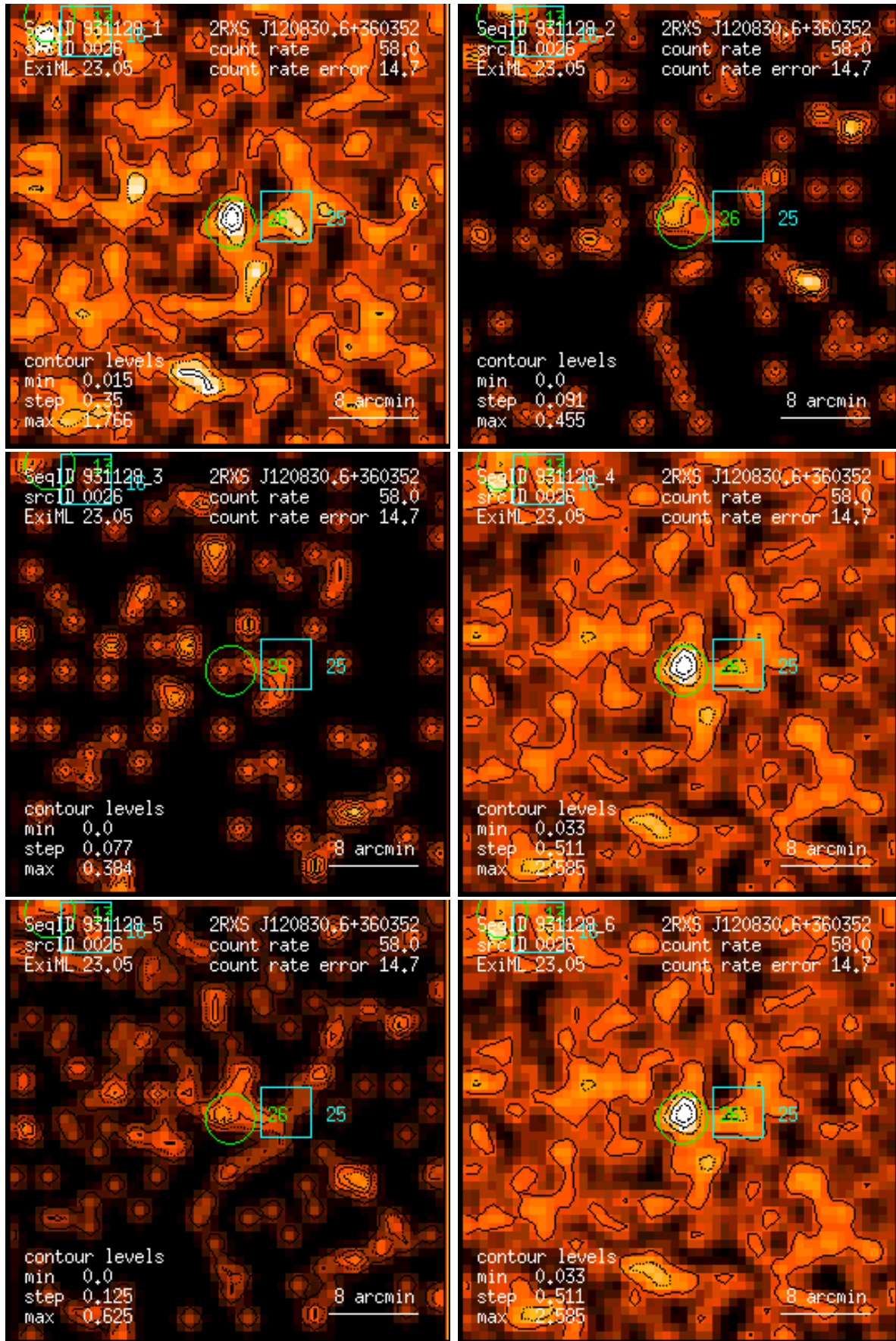
Figure 26: RASS 931128: detection 0026: band rate images, Gaussian filter: (1) PSPC channels 11 – 41, (2) 52 – 90, (3) 91 – 201, (4) 11 – 235, (5) 52 – 201, (6) 11 – 201. Broad band rates in counts/ks. Band rate contour levels in counts/ks/arcmin 2 .
