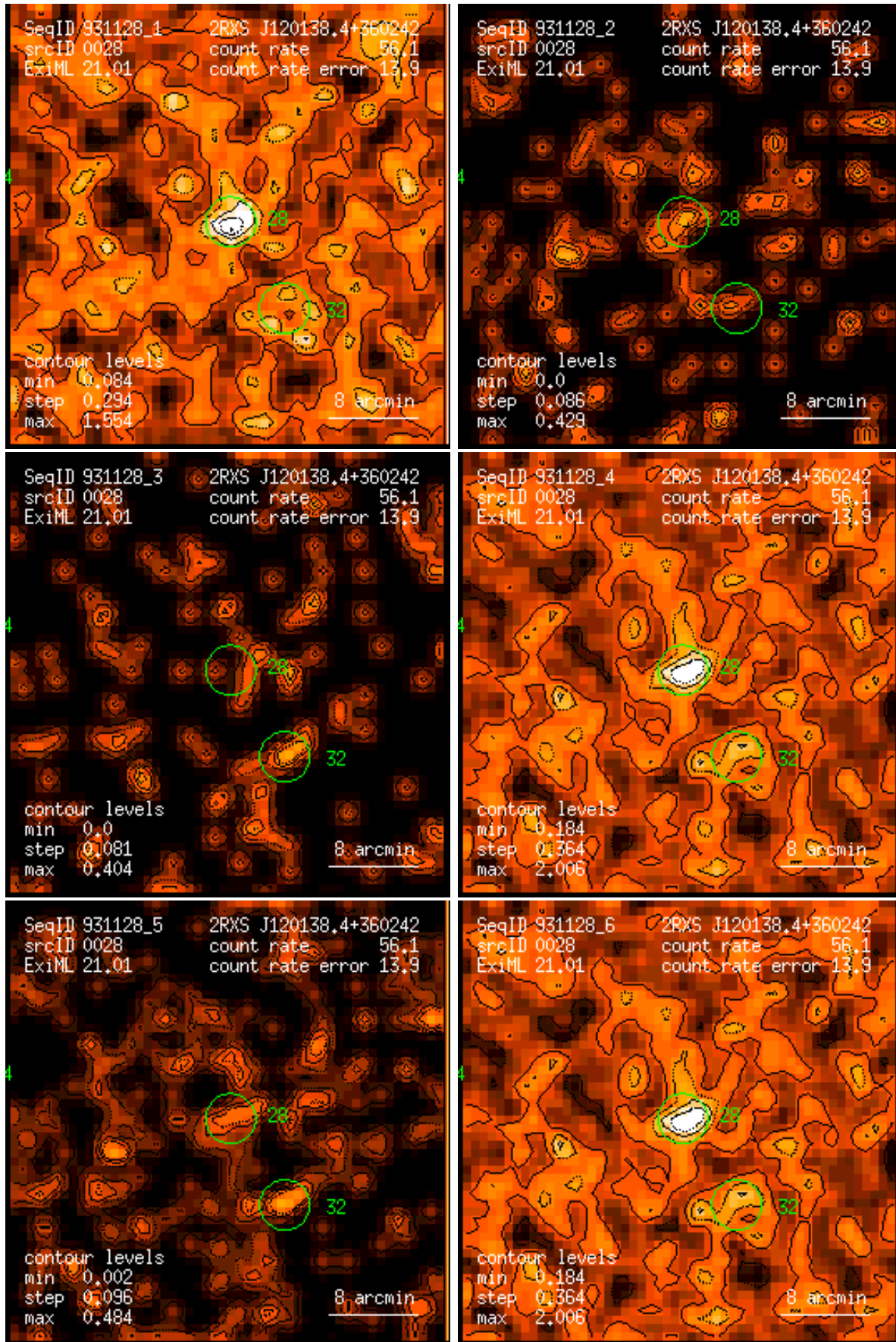
Figure 28: RASS 931128: detection 0028: band rate images, Gaussian filter: (1) PSPC channels 11 – 41, (2) 52 – 90, (3) 91 – 201, (4) 11 – 235, (5) 52 – 201, (6) 11 – 201. Broad band rates in counts/ks. Band rate contour levels in counts/ks/arcmin 2 .
