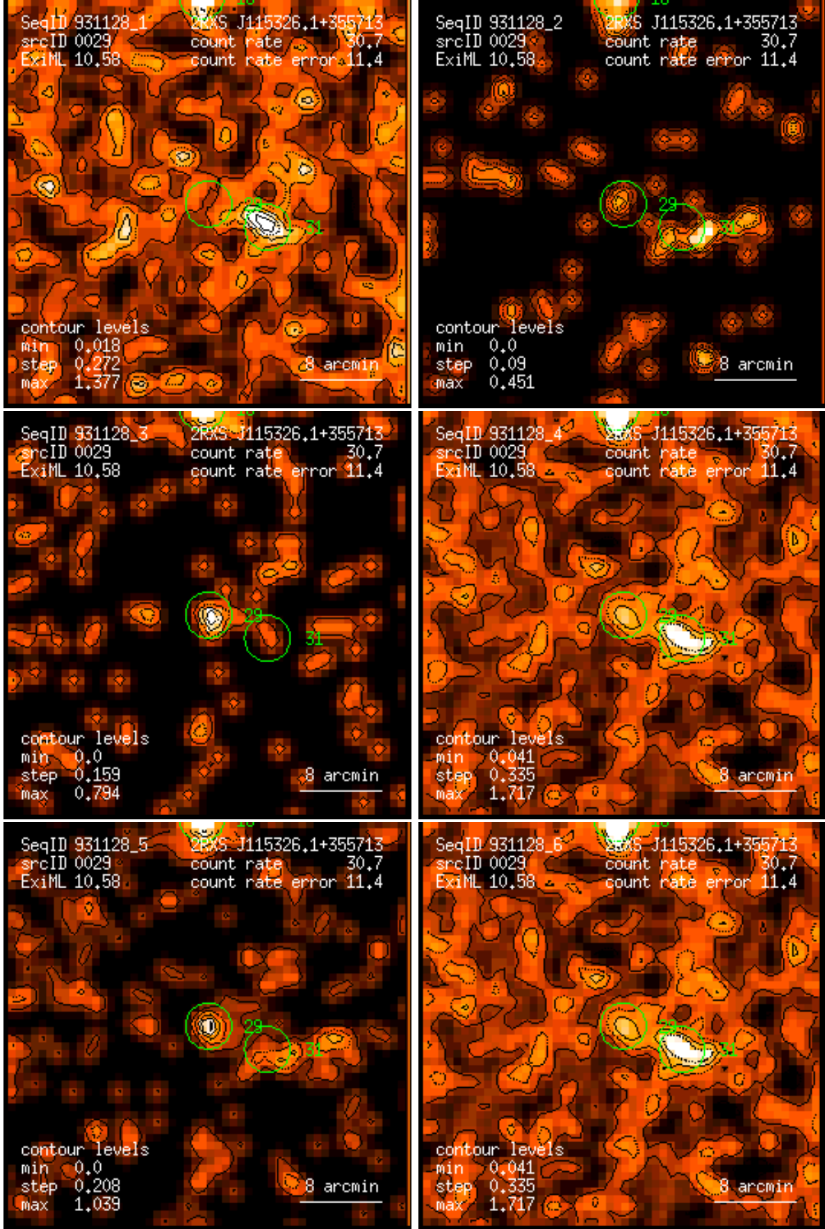
Figure 29: RASS 931128: detection 0029: band rate images, Gaussian filter: (1) PSPC channels 11 – 41, (2) 52 – 90, (3) 91 – 201, (4) 11 – 235, (5) 52 – 201, (6) 11 – 201. Broad band rates in counts/ks. Band rate contour levels in counts/ks/arcmin 2 .
