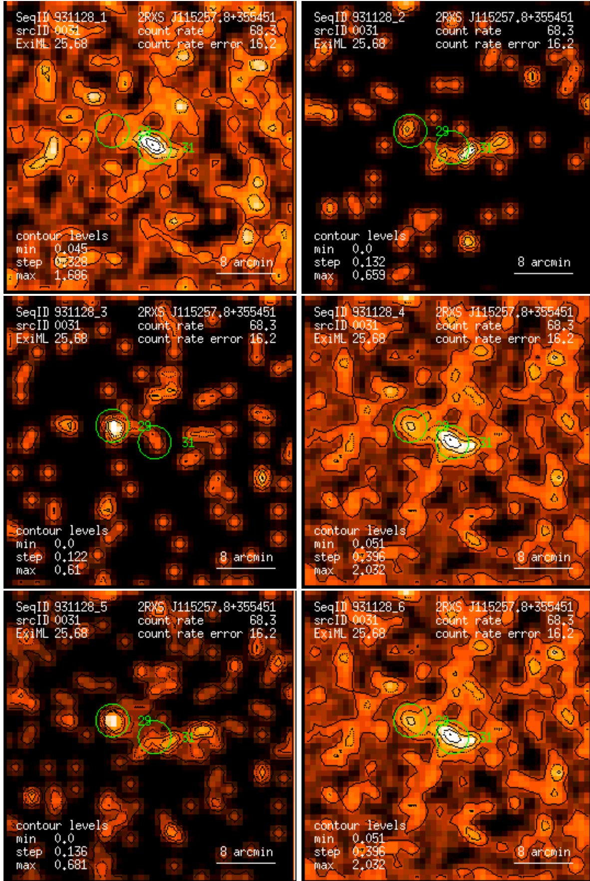
Figure 31: RASS 931128: detection 0031: band rate images, Gaussian filter: (1) PSPC channels 11 – 41, (2) 52 – 90, (3) 91 – 201, (4) 11 – 235, (5) 52 – 201, (6) 11 – 201. Broad band rates in counts/ks. Band rate contour levels in counts/ks/arcmin 2 .
