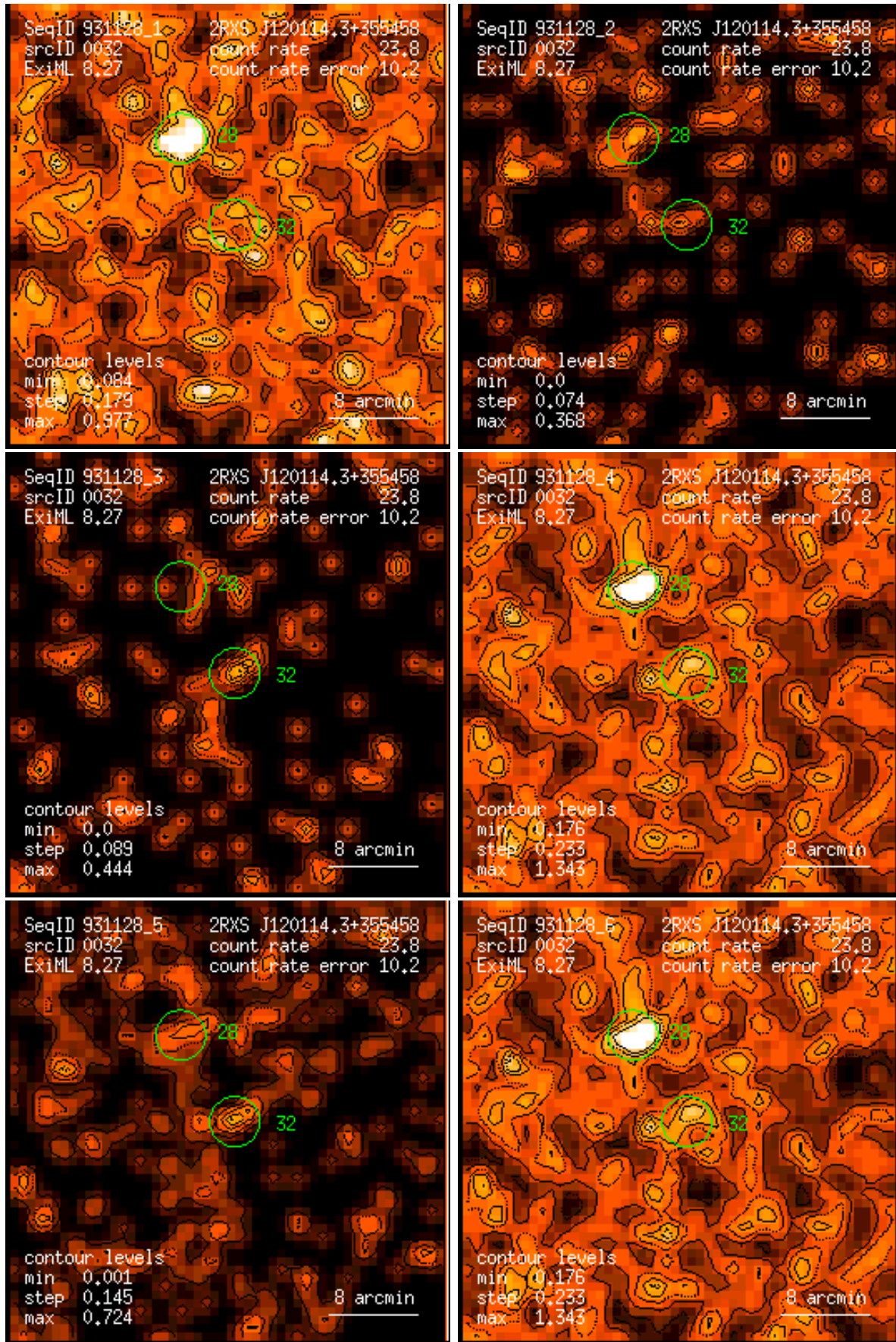
Figure 32: RASS 931128: detection 0032: band rate images, Gaussian filter: (1) PSPC channels 11 – 41, (2) 52 – 90, (3) 91 – 201, (4) 11 – 235, (5) 52 – 201, (6) 11 – 201. Broad band rates in counts/ks. Band rate contour levels in counts/ks/arcmin 2 .
