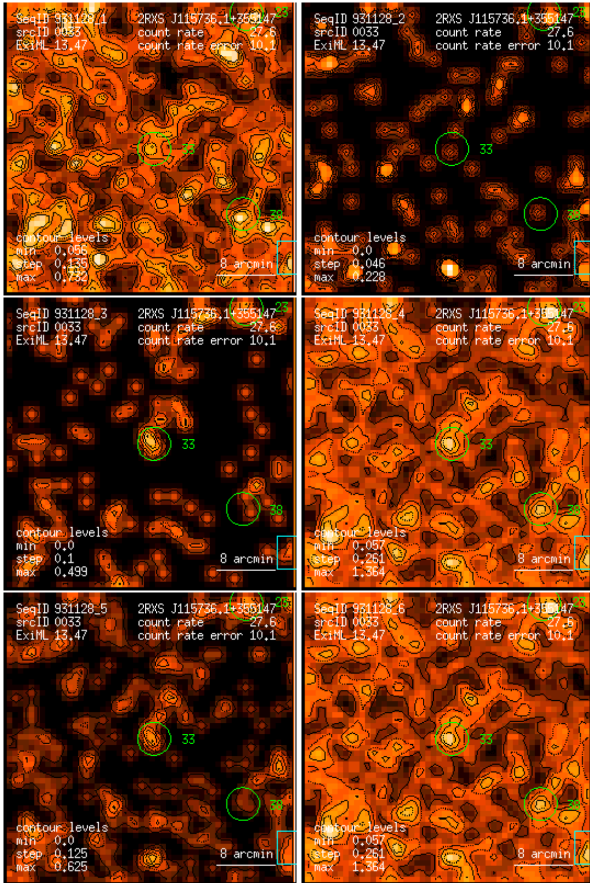
Figure 33: RASS 931128: detection 0033: band rate images, Gaussian filter: (1) PSPC channels 11 – 41, (2) 52 – 90, (3) 91 – 201, (4) 11 – 235, (5) 52 – 201, (6) 11 – 201. Broad band rates in counts/ks. Band rate contour levels in counts/ks/arcmin 2 .
