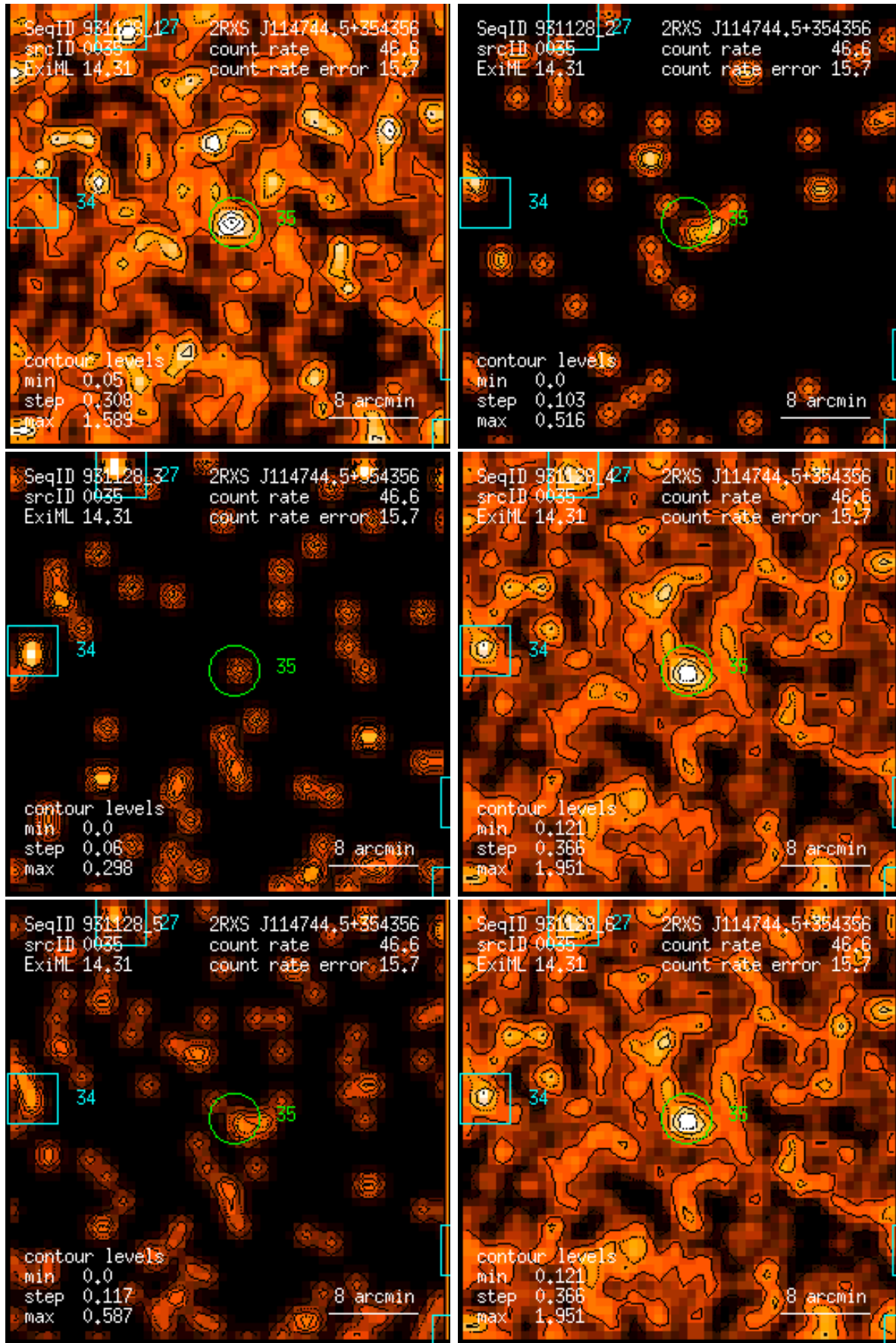
Figure 35: RASS 931128: detection 0035: band rate images, Gaussian filter: (1) PSPC channels 11 – 41, (2) 52 – 90, (3) 91 – 201, (4) 11 – 235, (5) 52 – 201, (6) 11 – 201. Broad band rates in counts/ks. Band rate contour levels in counts/ks/arcmin 2 .
