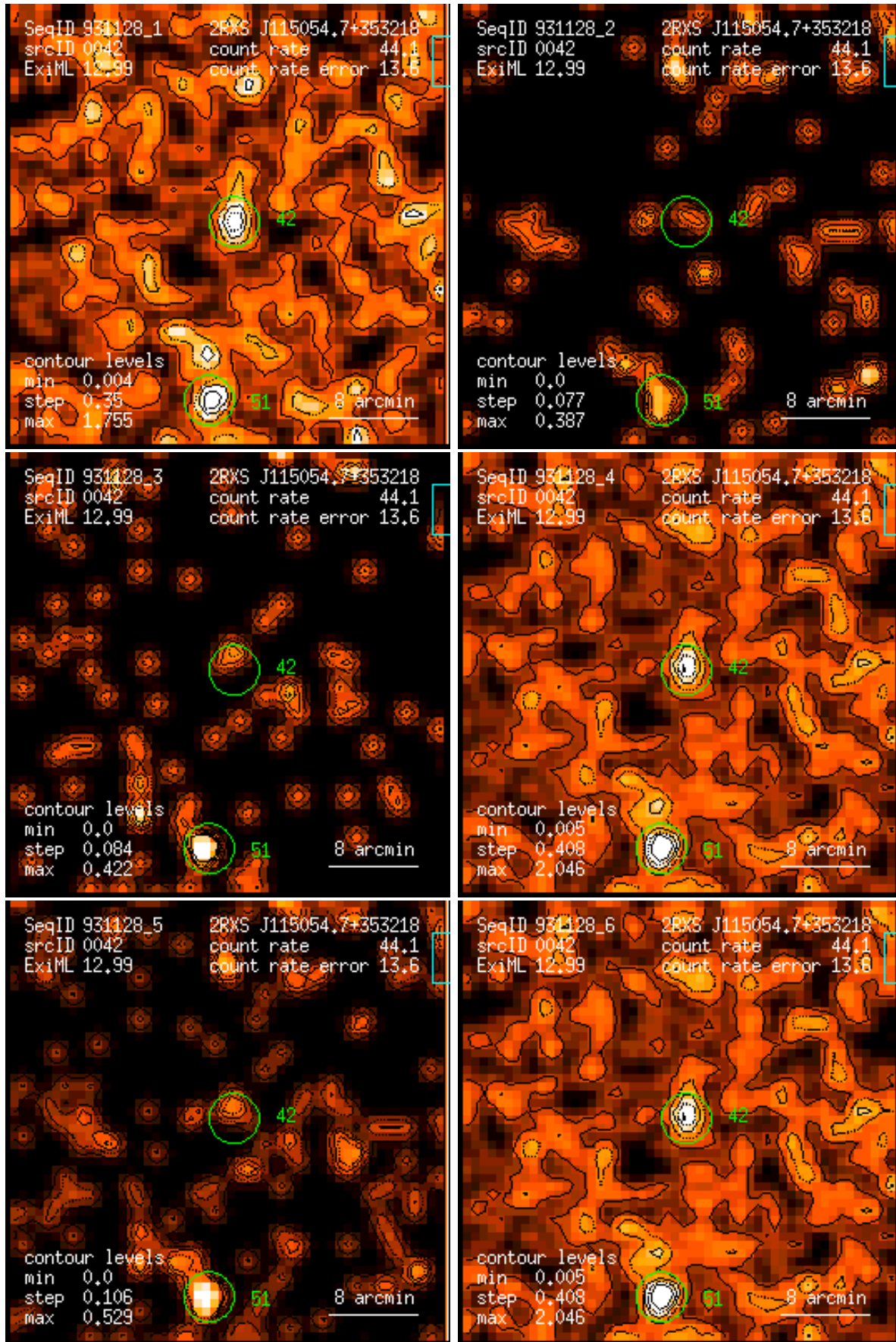
Figure 42: RASS 931128: detection 0042: band rate images, Gaussian filter: (1) PSPC channels 11 – 41, (2) 52 – 90, (3) 91 – 201, (4) 11 – 235, (5) 52 – 201, (6) 11 – 201. Broad band rates in counts/ks. Band rate contour levels in counts/ks/arcmin 2 .
