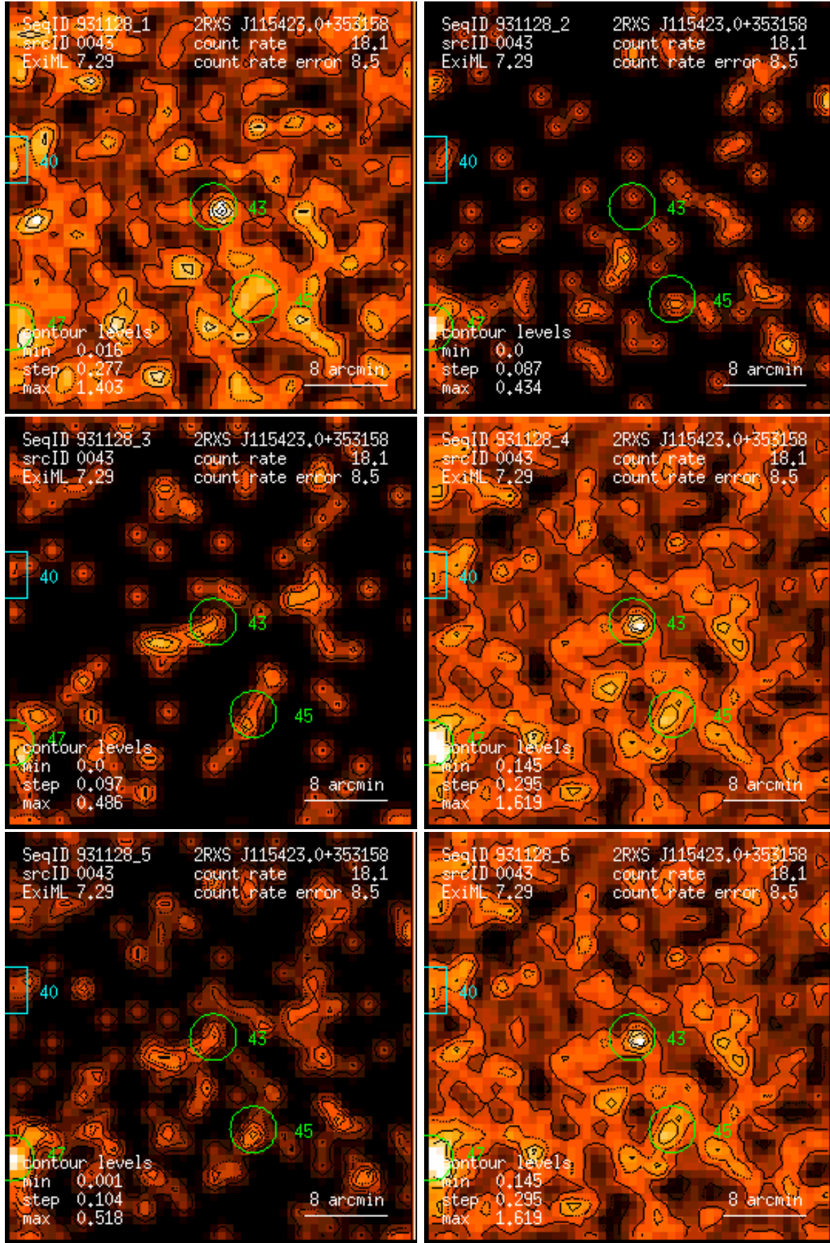
Figure 43: RASS 931128: detection 0043: band rate images, Gaussian filter: (1) PSPC channels 11 – 41, (2) 52 – 90, (3) 91 – 201, (4) 11 – 235, (5) 52 – 201, (6) 11 – 201. Broad band rates in counts/ks. Band rate contour levels in counts/ks/arcmin 2 .
