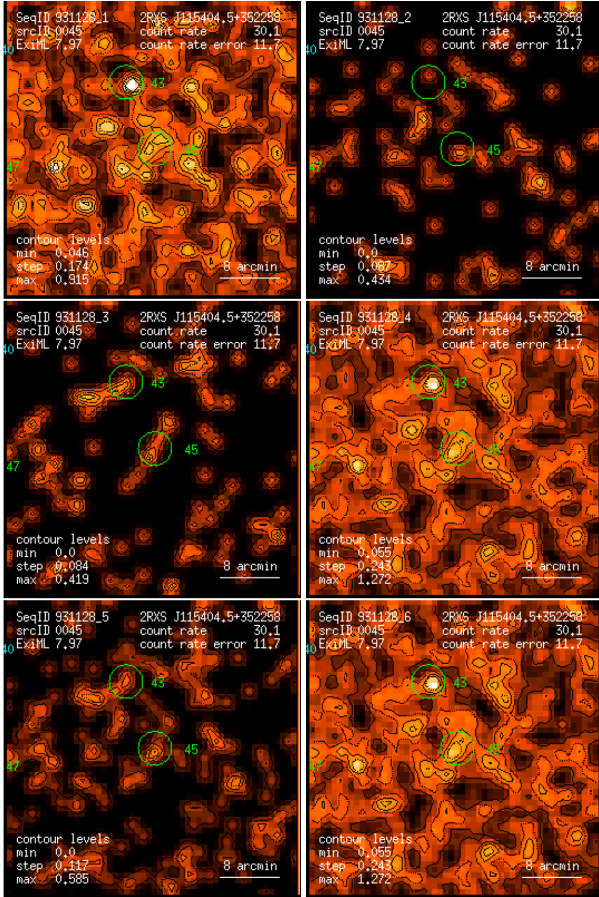
Figure 45: RASS 931128: detection 0045: band rate images, Gaussian filter: (1) PSPC channels 11 – 41, (2) 52 – 90, (3) 91 – 201, (4) 11 – 235, (5) 52 – 201, (6) 11 – 201. Broad band rates in counts/ks. Band rate contour levels in counts/ks/arcmin 2 .
