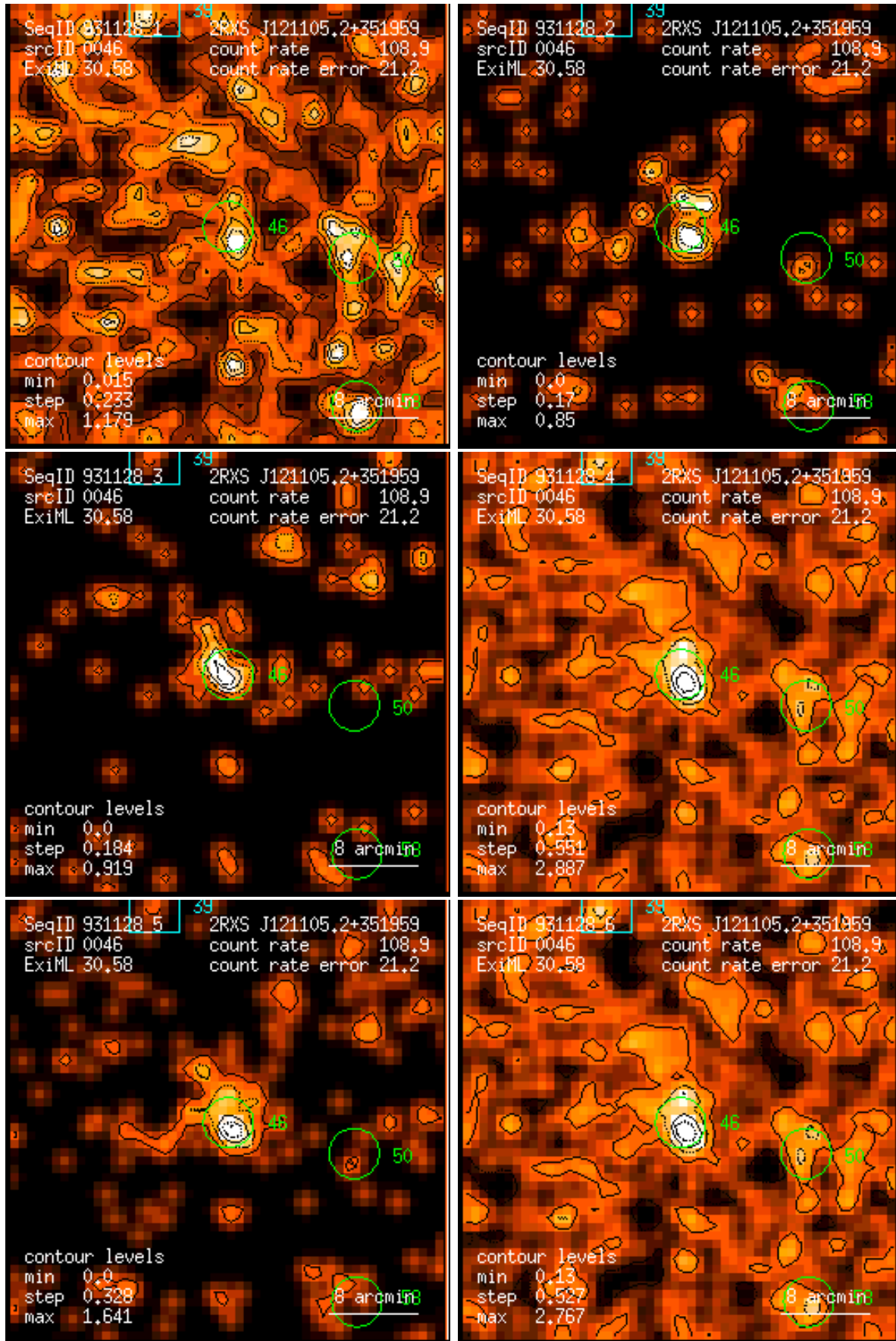
Figure 46: RASS 931128: detection 0046: band rate images, Gaussian filter: (1) PSPC channels 11 – 41, (2) 52 – 90, (3) 91 – 201, (4) 11 – 235, (5) 52 – 201, (6) 11 – 201. Broad band rates in counts/ks. Band rate contour levels in counts/ks/arcmin 2 .
