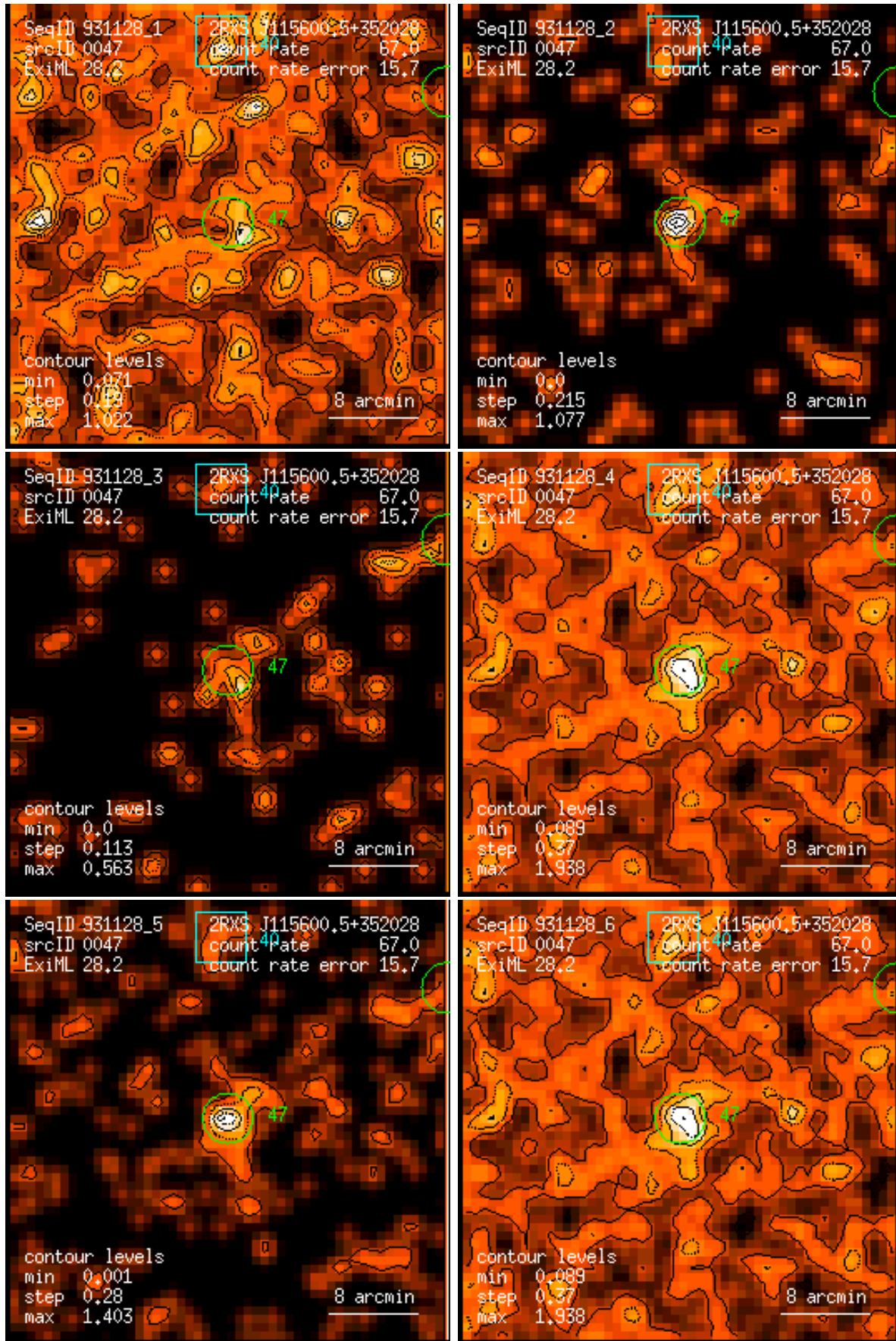
Figure 47: RASS 931128: detection 0047: band rate images, Gaussian filter: (1) PSPC channels 11 – 41, (2) 52 – 90, (3) 91 – 201, (4) 11 – 235, (5) 52 – 201, (6) 11 – 201. Broad band rates in counts/ks. Band rate contour levels in counts/ks/arcmin 2 .
