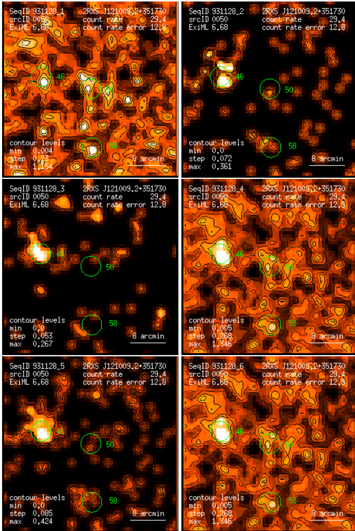
Figure 50: RASS 931128: detection 0050: band rate images, Gaussian filter: (1) PSPC channels 11 – 41, (2) 52 – 90, (3) 91 – 201, (4) 11 – 235, (5) 52 – 201, (6) 11 – 201. Broad band rates in counts/ks. Band rate contour levels in counts/ks/arcmin 2 .
