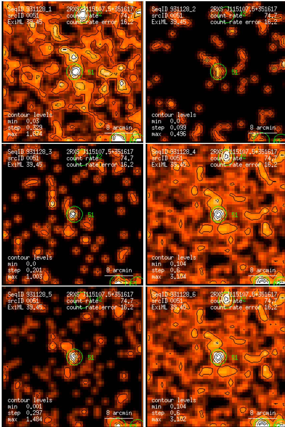
Figure 51: RASS 931128: detection 0051: band rate images, Gaussian filter: (1) PSPC channels 11 – 41, (2) 52 – 90, (3) 91 – 201, (4) 11 – 235, (5) 52 – 201, (6) 11 – 201. Broad band rates in counts/ks. Band rate contour levels in counts/ks/arcmin 2 .
