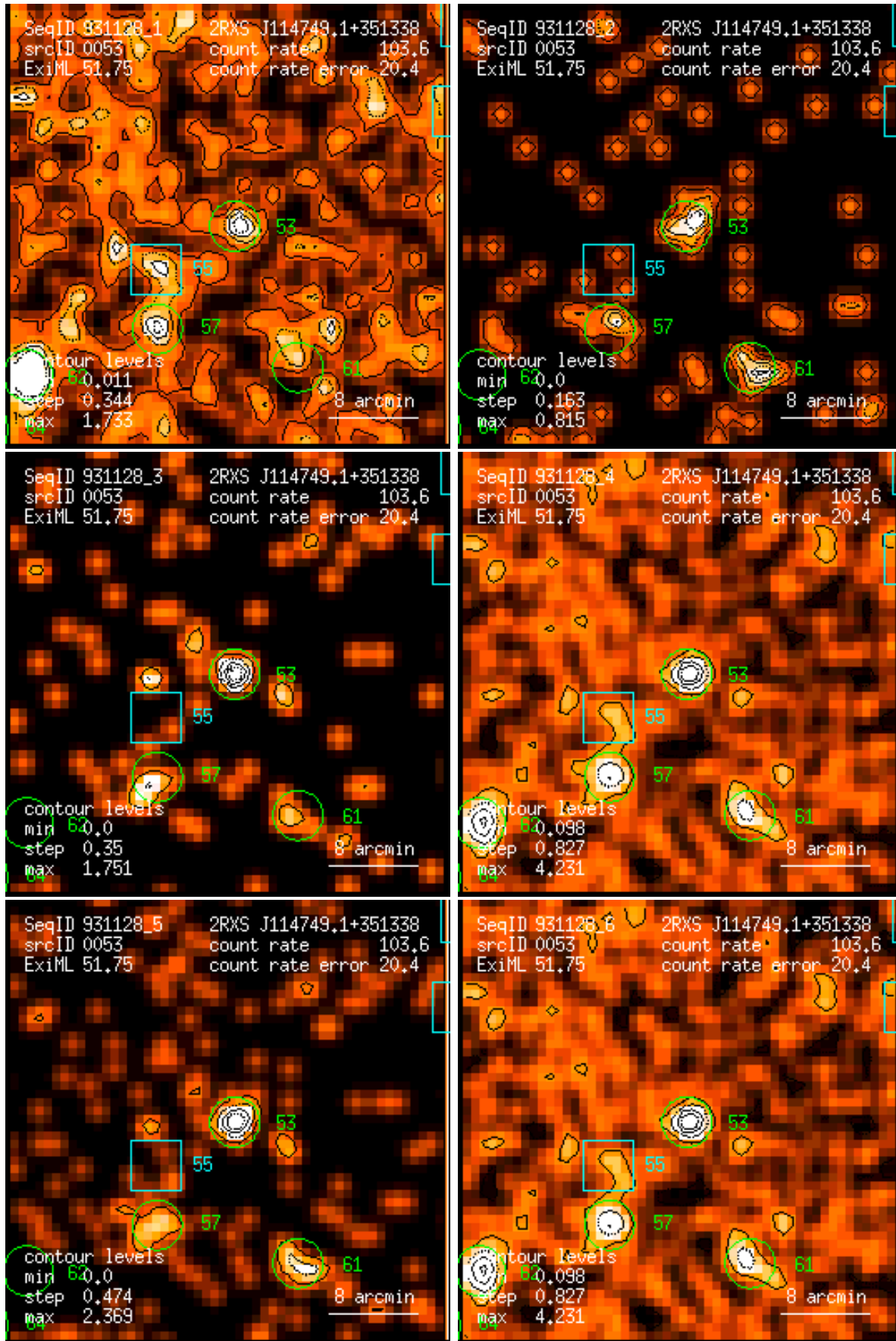
Figure 53: RASS 931128: detection 0053: band rate images, Gaussian filter: (1) PSPC channels 11 – 41, (2) 52 – 90, (3) 91 – 201, (4) 11 – 235, (5) 52 – 201, (6) 11 – 201. Broad band rates in counts/ks. Band rate contour levels in counts/ks/arcmin 2 .
