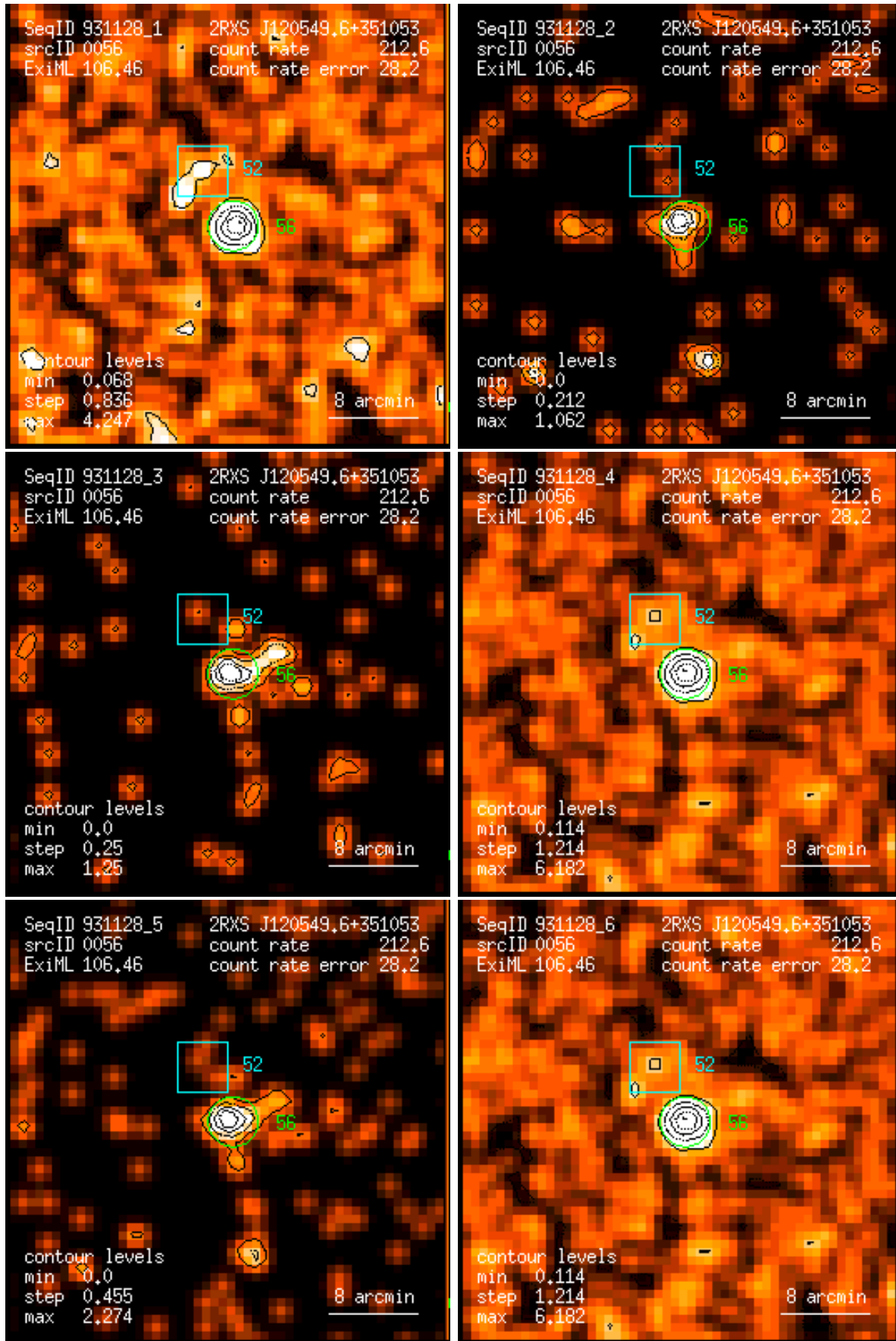
Figure 56: RASS 931128: detection 0056: band rate images, Gaussian filter: (1) PSPC channels 11 – 41, (2) 52 – 90, (3) 91 – 201, (4) 11 – 235, (5) 52 – 201, (6) 11 – 201. Broad band rates in counts/ks. Band rate contour levels in counts/ks/arcmin 2 .
