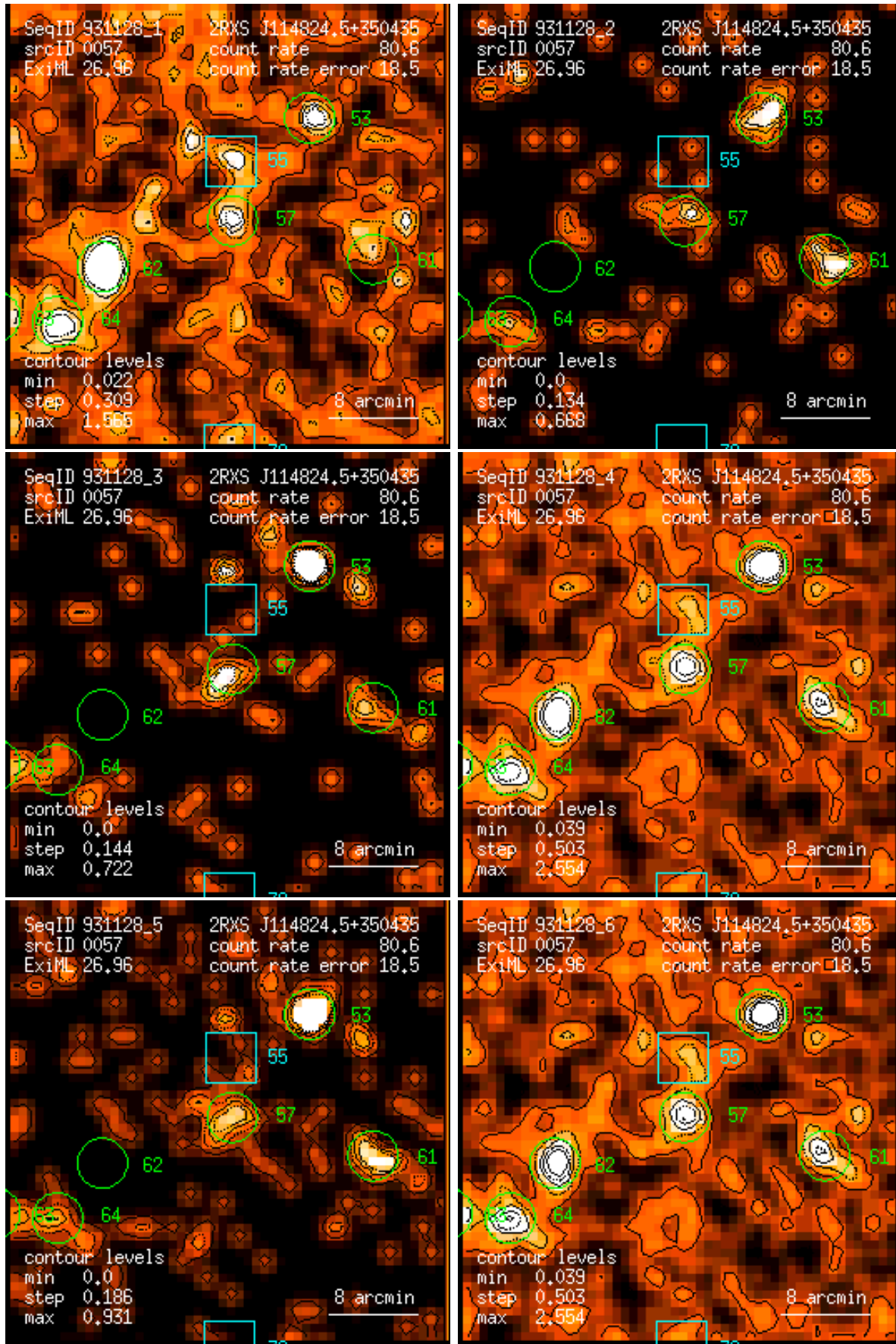
Figure 57: RASS 931128: detection 0057: band rate images, Gaussian filter: (1) PSPC channels 11 – 41, (2) 52 – 90, (3) 91 – 201, (4) 11 – 235, (5) 52 – 201, (6) 11 – 201. Broad band rates in counts/ks. Band rate contour levels in counts/ks/arcmin 2 .
