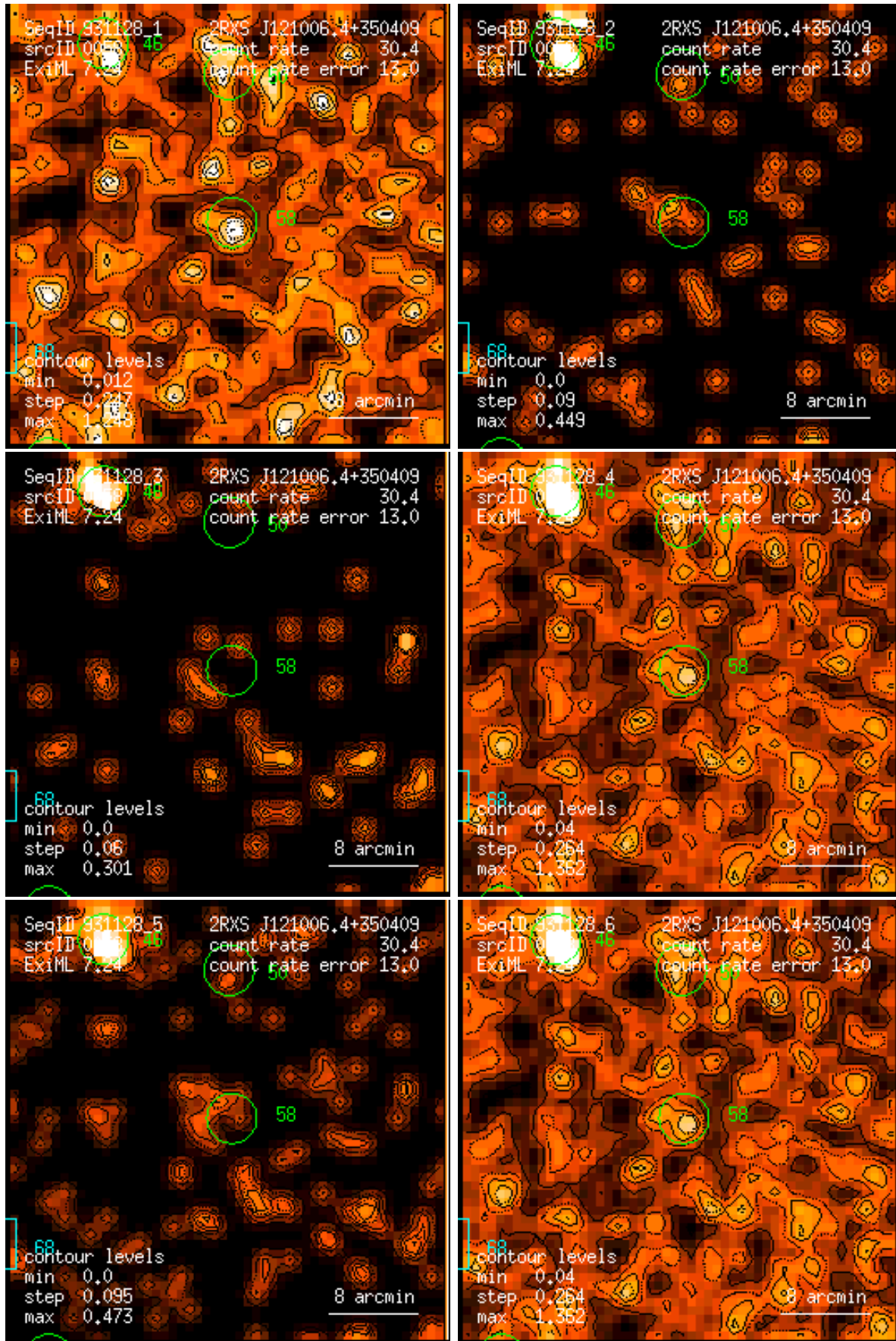
Figure 58: RASS 931128: detection 0058: band rate images, Gaussian filter: (1) PSPC channels 11 – 41, (2) 52 – 90, (3) 91 – 201, (4) 11 – 235, (5) 52 – 201, (6) 11 – 201. Broad band rates in counts/ks. Band rate contour levels in counts/ks/arcmin 2 .
