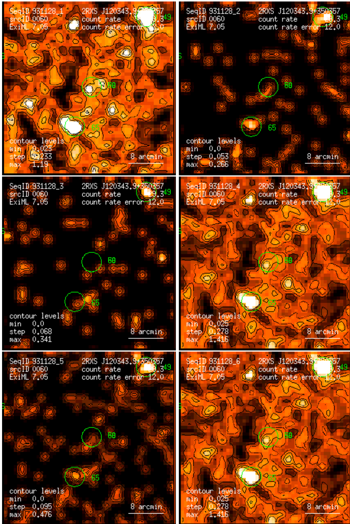
Figure 60: RASS 931128: detection 0060: band rate images, Gaussian filter: (1) PSPC channels 11 – 41, (2) 52 – 90, (3) 91 – 201, (4) 11 – 235, (5) 52 – 201, (6) 11 – 201. Broad band rates in counts/ks. Band rate contour levels in counts/ks/arcmin 2 .
