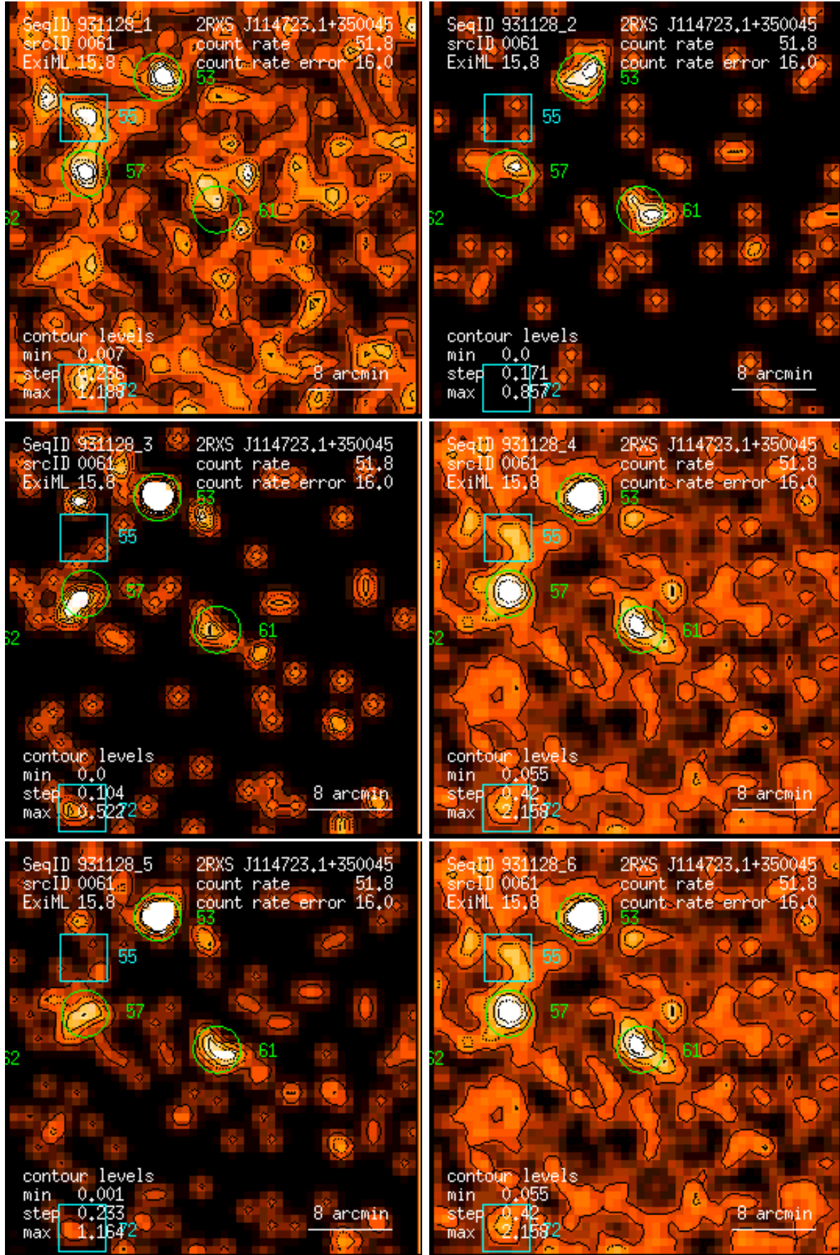
Figure 61: RASS 931128: detection 0061: band rate images, Gaussian filter: (1) PSPC channels 11 – 41, (2) 52 – 90, (3) 91 – 201, (4) 11 – 235, (5) 52 – 201, (6) 11 – 201. Broad band rates in counts/ks. Band rate contour levels in counts/ks/arcmin 2 .
