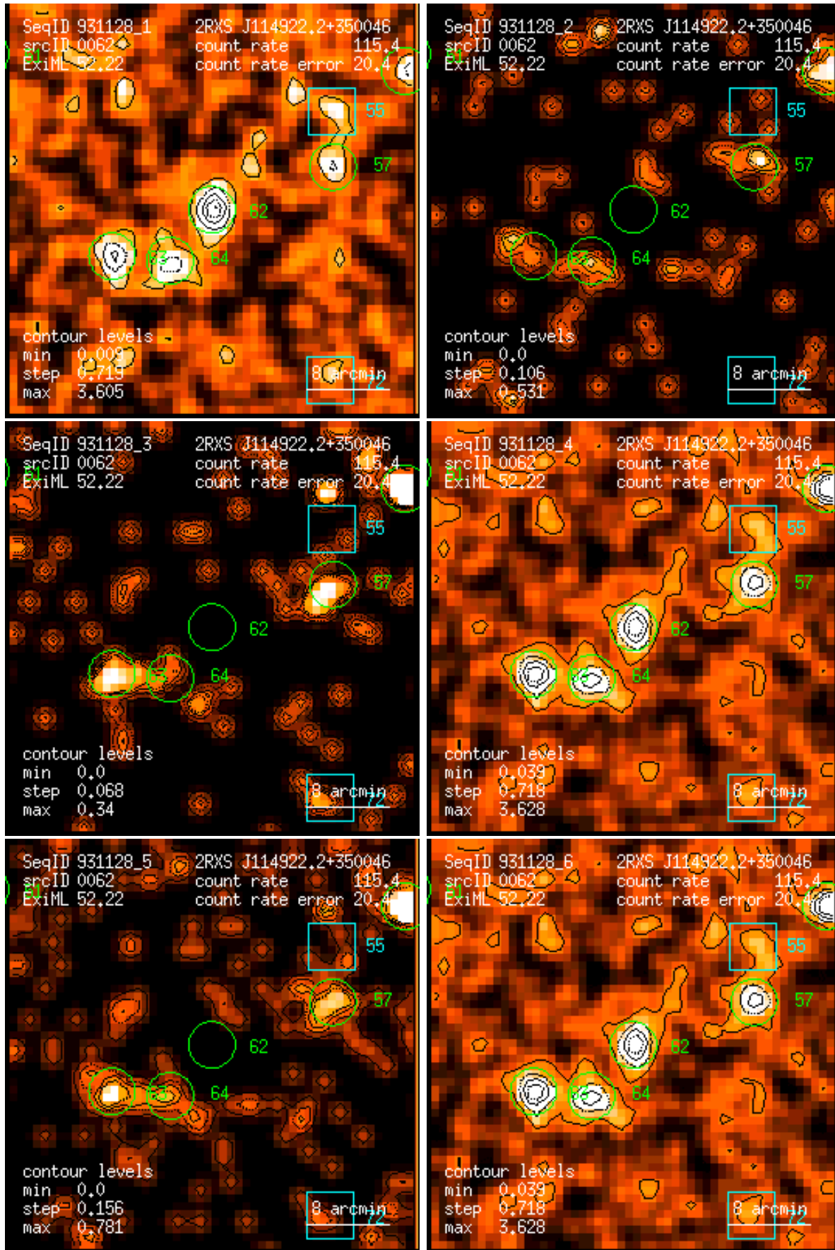
Figure 62: RASS 931128: detection 0062: band rate images, Gaussian filter: (1) PSPC channels 11 – 41, (2) 52 – 90, (3) 91 – 201, (4) 11 – 235, (5) 52 – 201, (6) 11 – 201. Broad band rates in counts/ks. Band rate contour levels in counts/ks/arcmin 2 .
