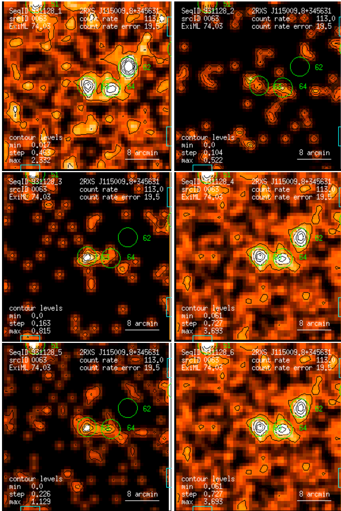
Figure 63: RASS 931128: detection 0063: band rate images, Gaussian filter: (1) PSPC channels 11 – 41, (2) 52 – 90, (3) 91 – 201, (4) 11 – 235, (5) 52 – 201, (6) 11 – 201. Broad band rates in counts/ks. Band rate contour levels in counts/ks/arcmin 2 .
