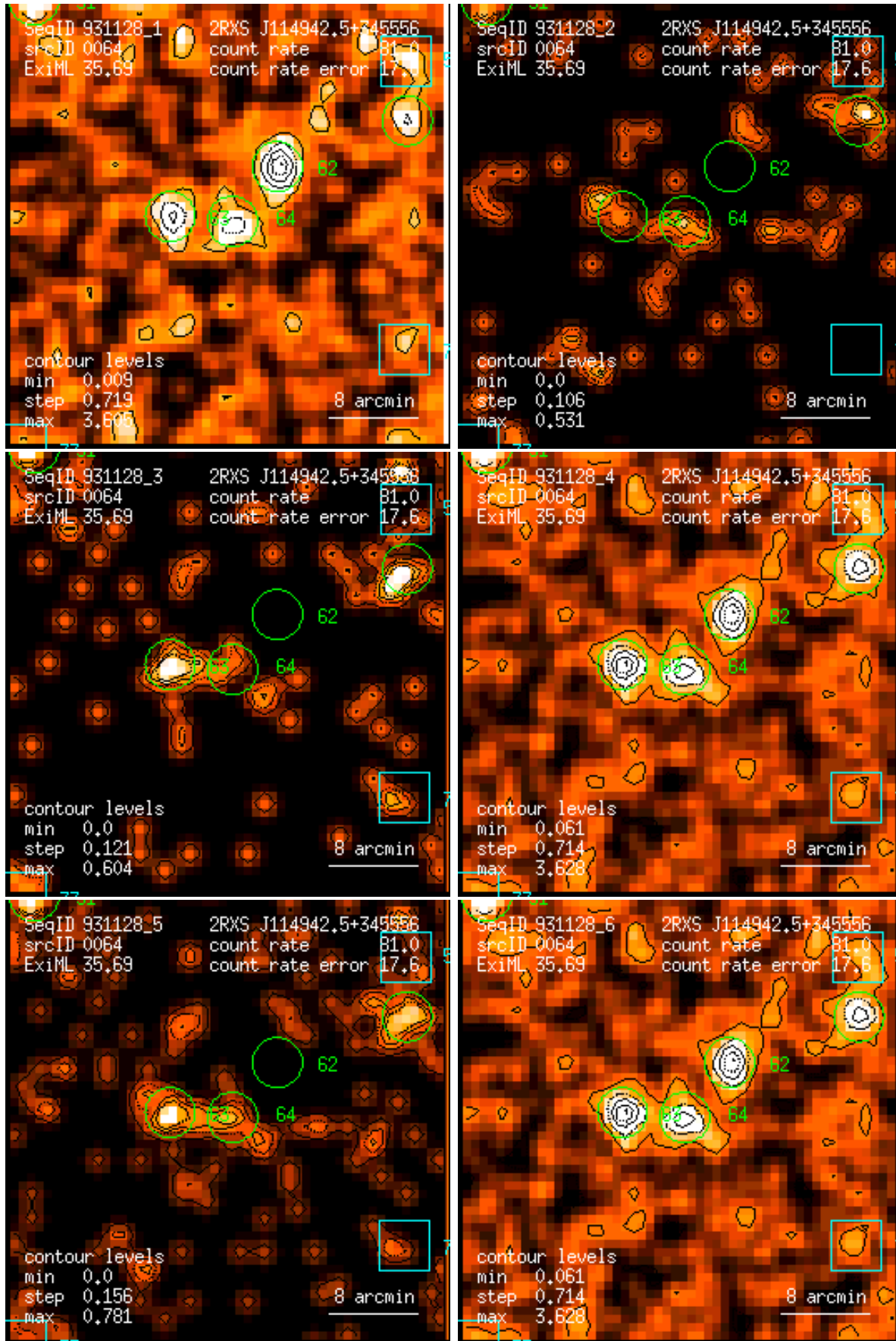
Figure 64: RASS 931128: detection 0064: band rate images, Gaussian filter: (1) PSPC channels 11 – 41, (2) 52 – 90, (3) 91 – 201, (4) 11 – 235, (5) 52 – 201, (6) 11 – 201. Broad band rates in counts/ks. Band rate contour levels in counts/ks/arcmin 2 .
