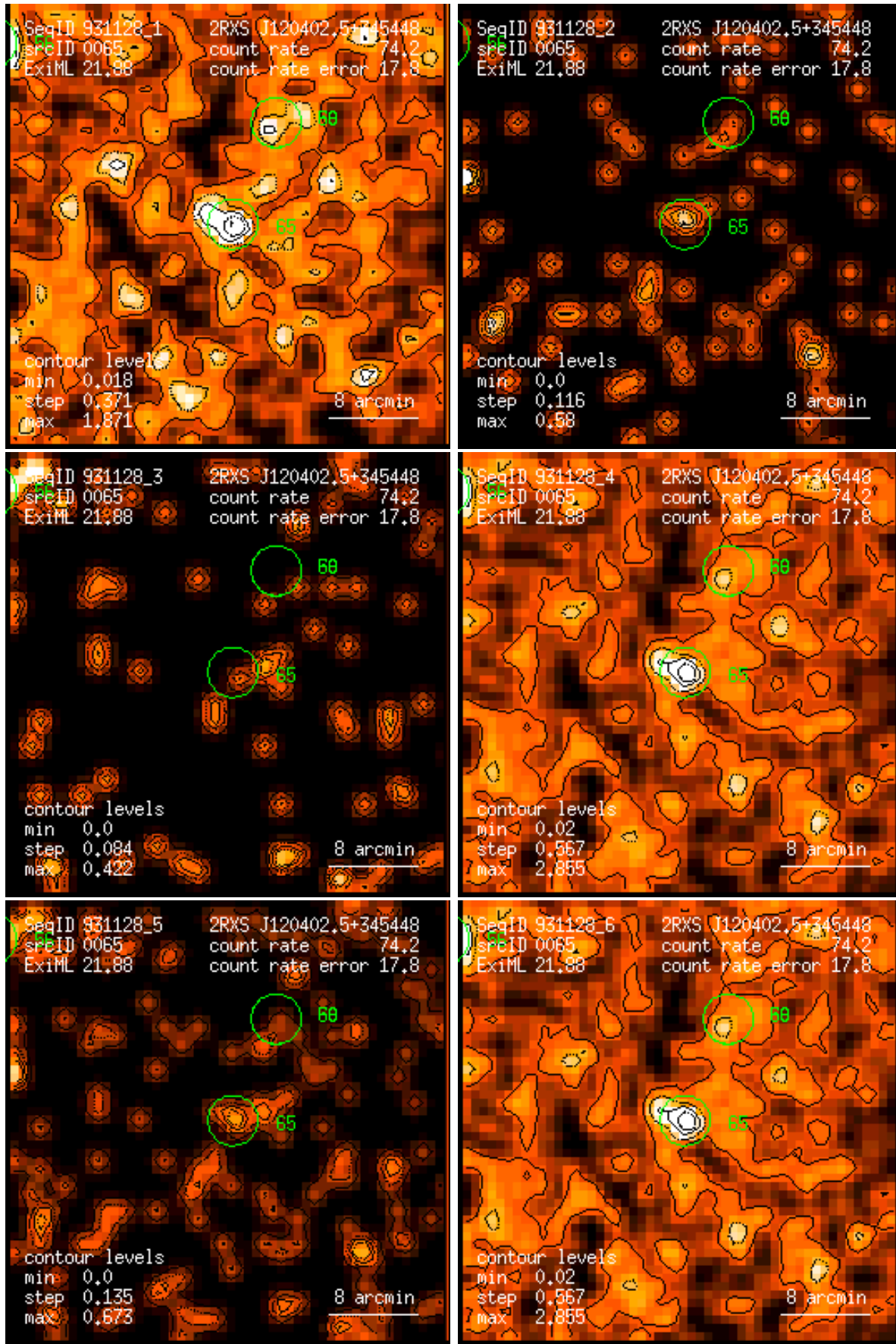
Figure 65: RASS 931128: detection 0065: band rate images, Gaussian filter: (1) PSPC channels 11 – 41, (2) 52 – 90, (3) 91 – 201, (4) 11 – 235, (5) 52 – 201, (6) 11 – 201. Broad band rates in counts/ks. Band rate contour levels in counts/ks/arcmin 2 .
