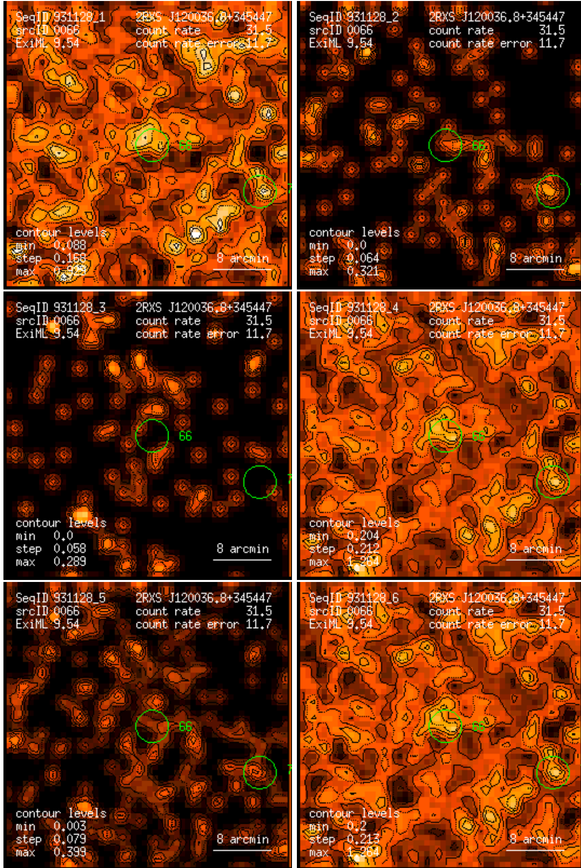
Figure 66: RASS 931128: detection 0066: band rate images, Gaussian filter: (1) PSPC channels 11 – 41, (2) 52 – 90, (3) 91 – 201, (4) 11 – 235, (5) 52 – 201, (6) 11 – 201. Broad band rates in counts/ks. Band rate contour levels in counts/ks/arcmin 2 .
