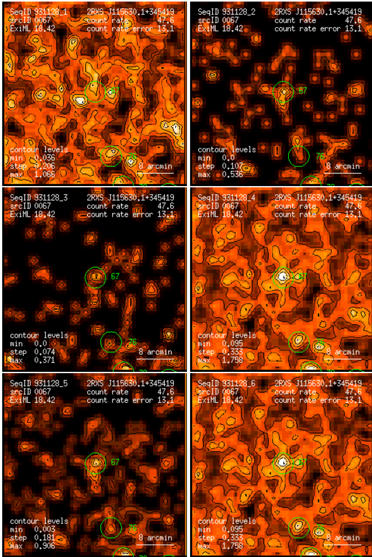
Figure 67: RASS 931128: detection 0067: band rate images, Gaussian filter: (1) PSPC channels 11 – 41, (2) 52 – 90, (3) 91 – 201, (4) 11 – 235, (5) 52 – 201, (6) 11 – 201. Broad band rates in counts/ks. Band rate contour levels in counts/ks/arcmin 2 .
