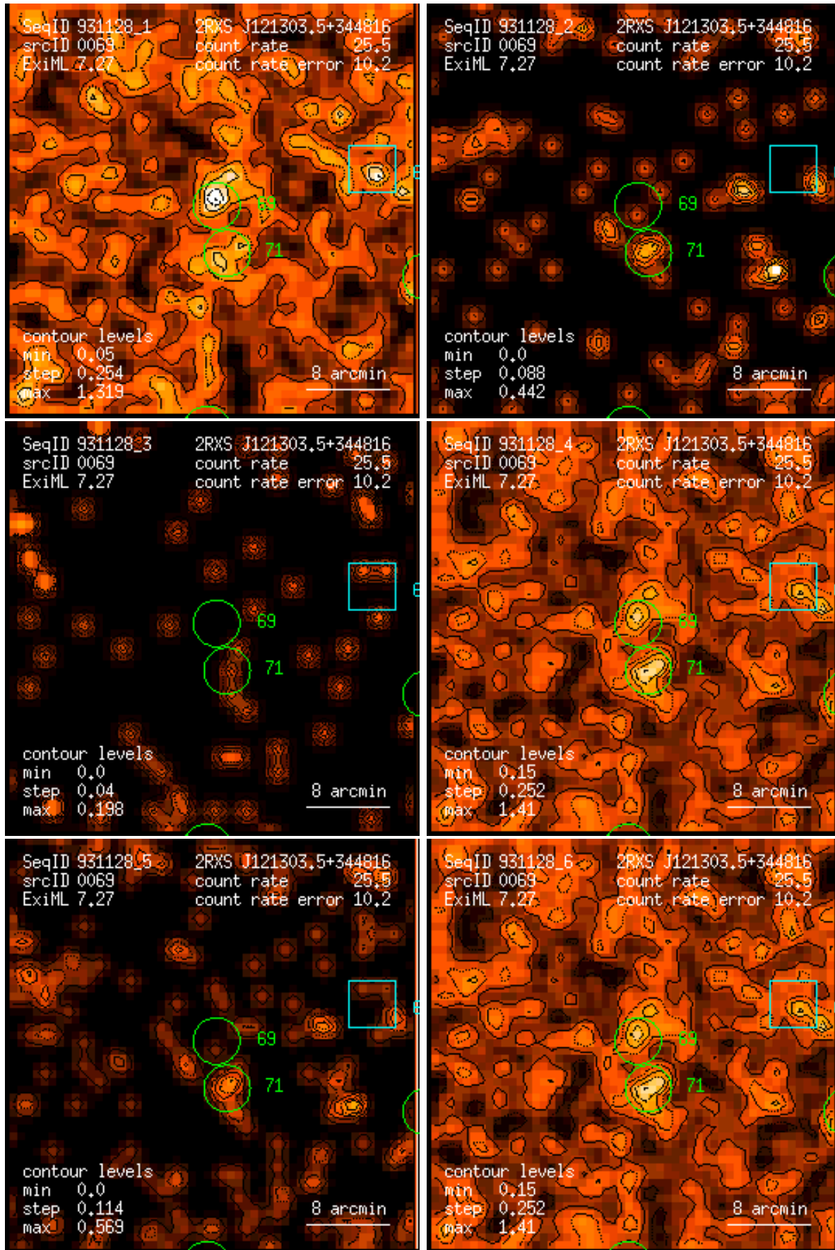
Figure 69: RASS 931128: detection 0069: band rate images, Gaussian filter: (1) PSPC channels 11 – 41, (2) 52 – 90, (3) 91 – 201, (4) 11 – 235, (5) 52 – 201, (6) 11 – 201. Broad band rates in counts/ks. Band rate contour levels in counts/ks/arcmin 2 .
