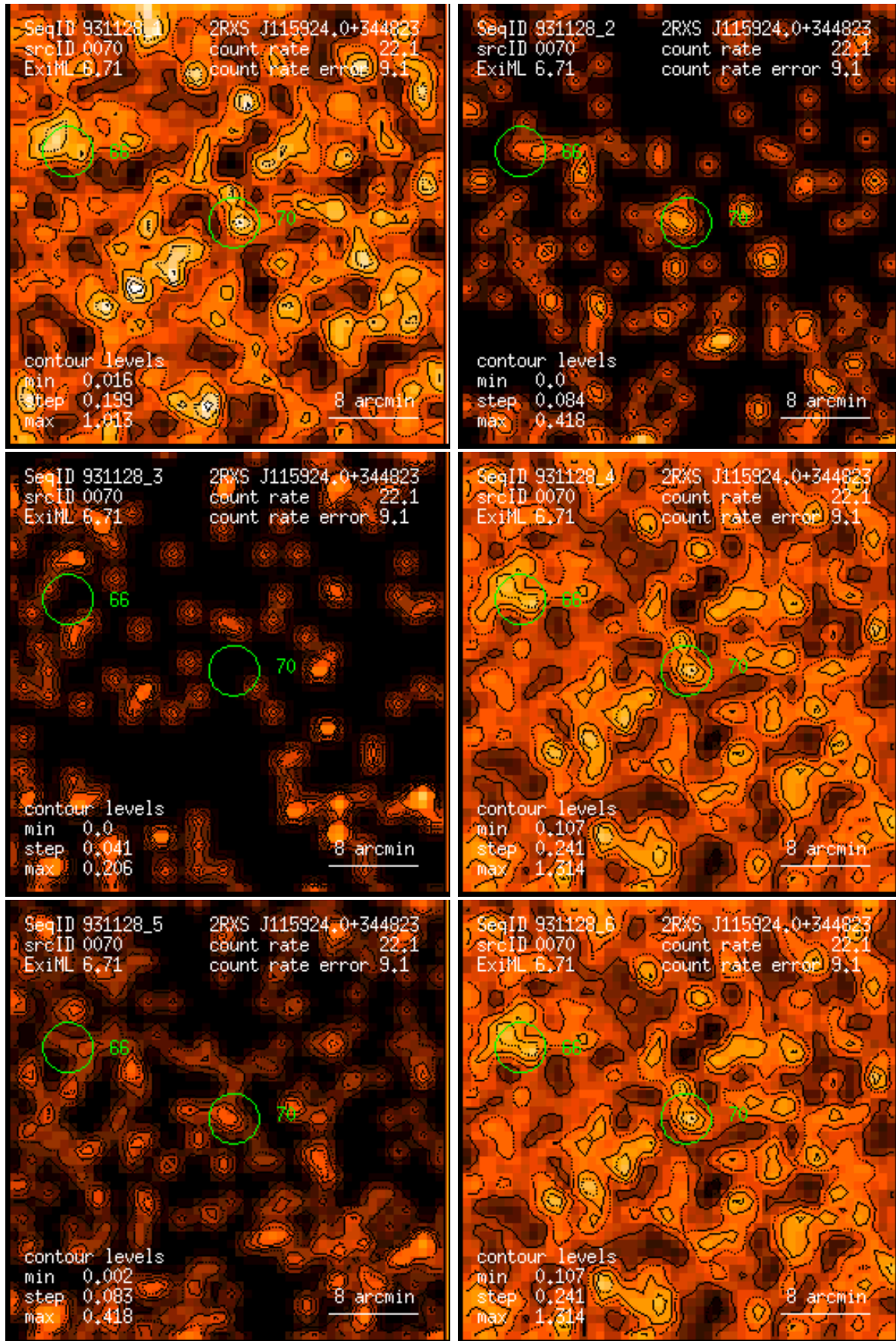
Figure 70: RASS 931128: detection 0070: band rate images, Gaussian filter: (1) PSPC channels 11 – 41, (2) 52 – 90, (3) 91 – 201, (4) 11 – 235, (5) 52 – 201, (6) 11 – 201. Broad band rates in counts/ks. Band rate contour levels in counts/ks/arcmin 2 .
