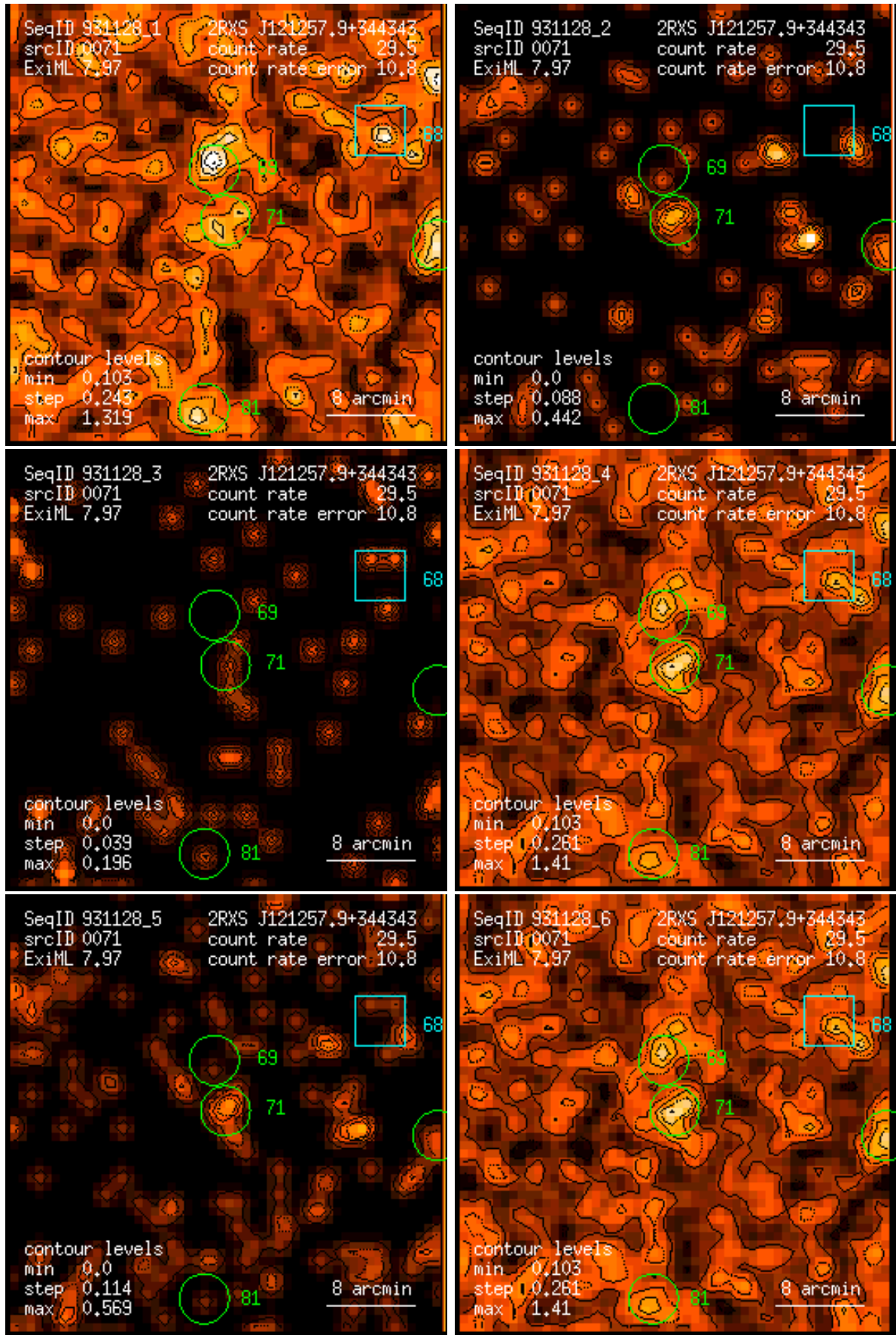
Figure 71: RASS 931128: detection 0071: band rate images, Gaussian filter: (1) PSPC channels 11 – 41, (2) 52 – 90, (3) 91 – 201, (4) 11 – 235, (5) 52 – 201, (6) 11 – 201. Broad band rates in counts/ks. Band rate contour levels in counts/ks/arcmin 2 .
