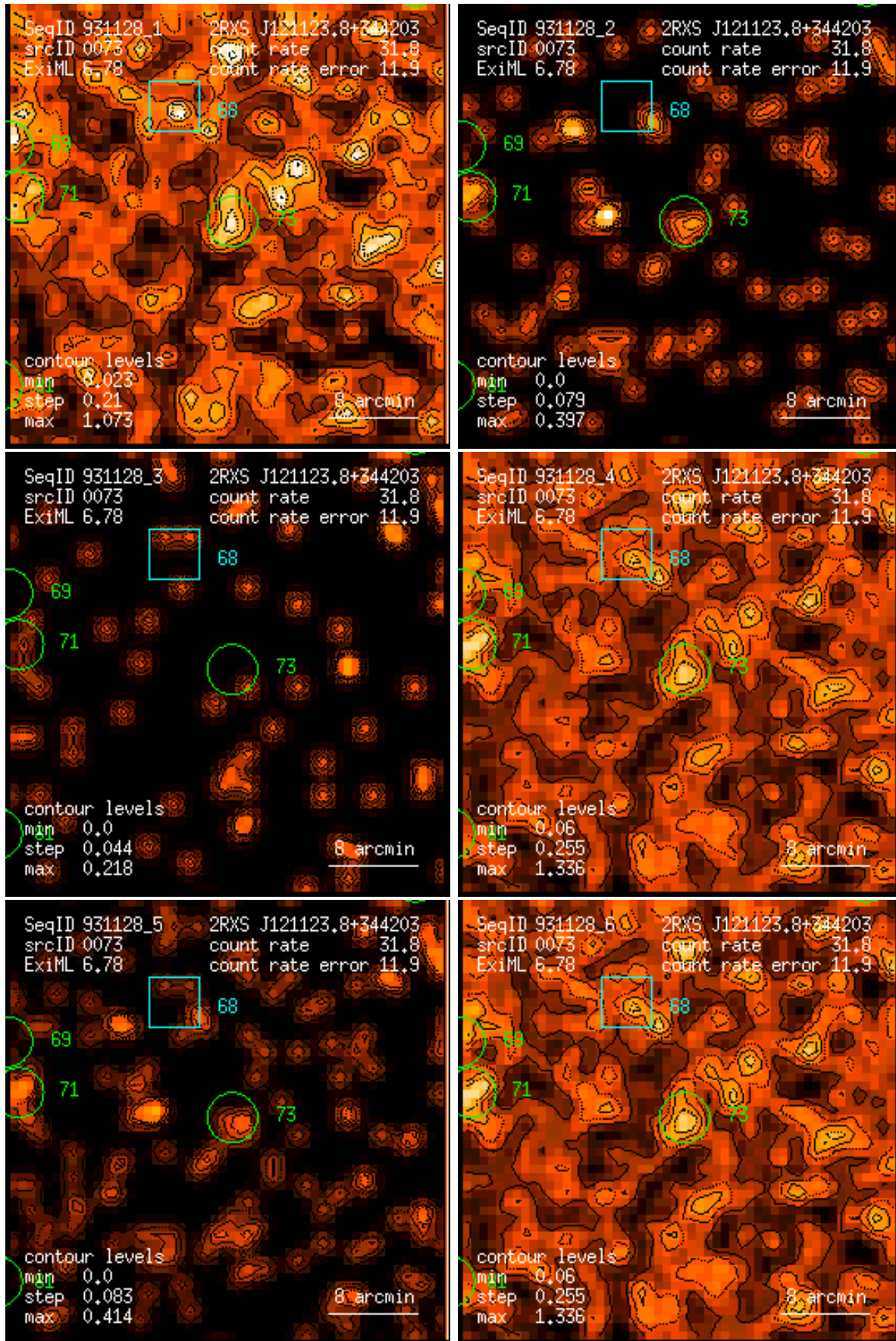
Figure 73: RASS 931128: detection 0073: band rate images, Gaussian filter: (1) PSPC channels 11 – 41, (2) 52 – 90, (3) 91 – 201, (4) 11 – 235, (5) 52 – 201, (6) 11 – 201. Broad band rates in counts/ks. Band rate contour levels in counts/ks/arcmin 2 .
