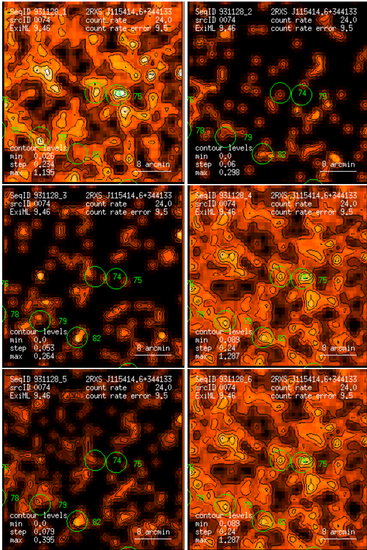
Figure 74: RASS 931128: detection 0074: band rate images, Gaussian filter: (1) PSPC channels 11 – 41, (2) 52 – 90, (3) 91 – 201, (4) 11 – 235, (5) 52 – 201, (6) 11 – 201. Broad band rates in counts/ks. Band rate contour levels in counts/ks/arcmin 2 .
