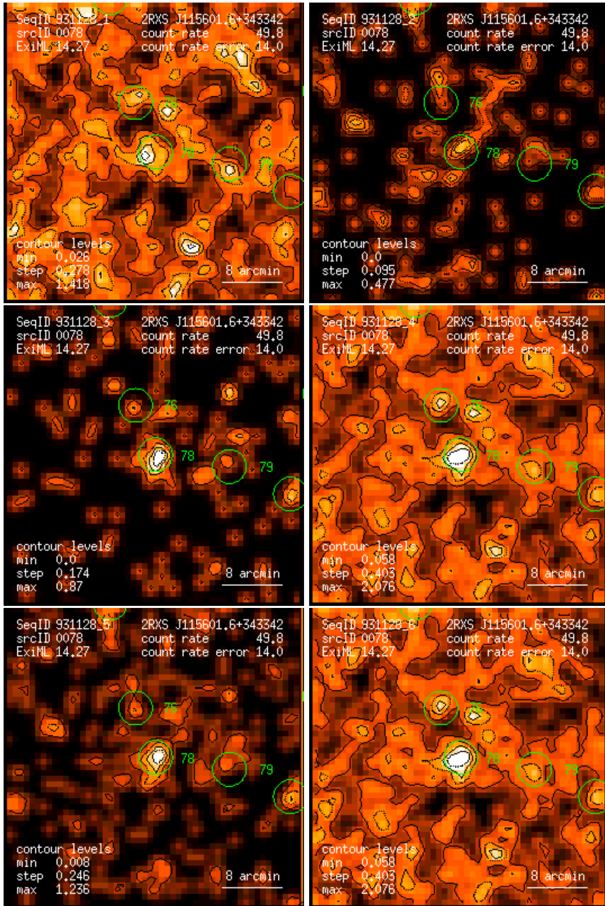
Figure 78: RASS 931128: detection 0078: band rate images, Gaussian filter: (1) PSPC channels 11 – 41, (2) 52 – 90, (3) 91 – 201, (4) 11 – 235, (5) 52 – 201, (6) 11 – 201. Broad band rates in counts/ks. Band rate contour levels in counts/ks/arcmin 2 .
