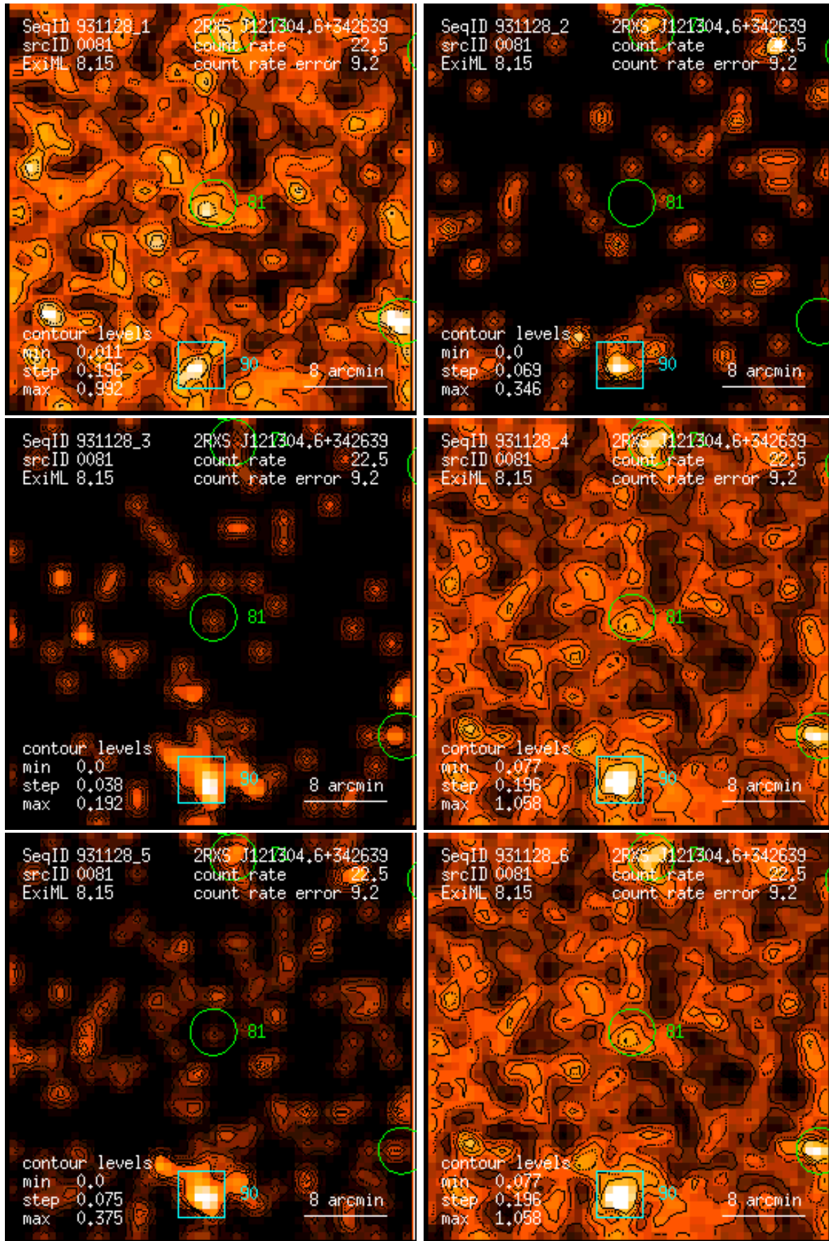
Figure 81: RASS 931128: detection 0081: band rate images, Gaussian filter: (1) PSPC channels 11 – 41, (2) 52 – 90, (3) 91 – 201, (4) 11 – 235, (5) 52 – 201, (6) 11 – 201. Broad band rates in counts/ks. Band rate contour levels in counts/ks/arcmin 2 .
