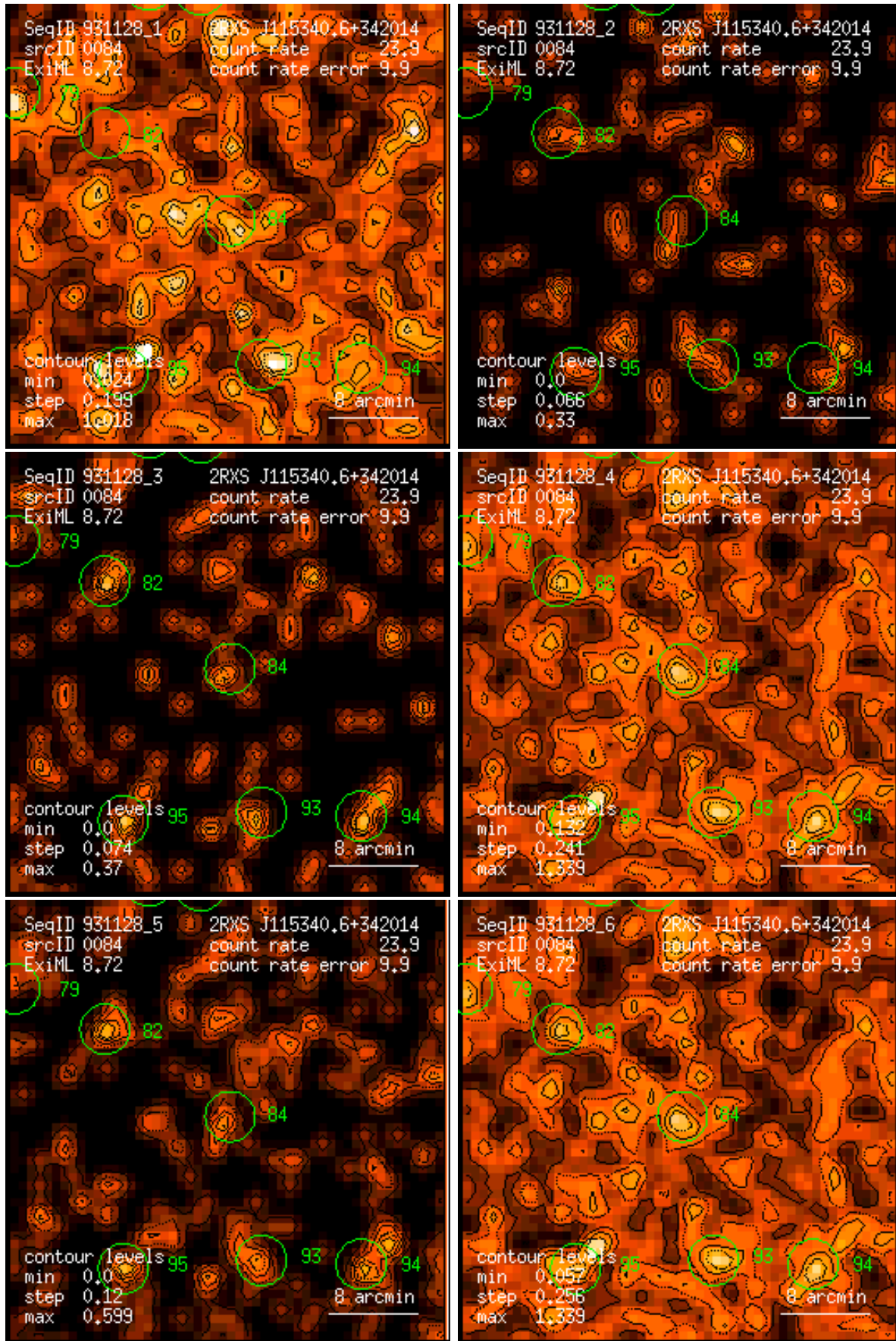
Figure 84: RASS 931128: detection 0084: band rate images, Gaussian filter: (1) PSPC channels 11 – 41, (2) 52 – 90, (3) 91 – 201, (4) 11 – 235, (5) 52 – 201, (6) 11 – 201. Broad band rates in counts/ks. Band rate contour levels in counts/ks/arcmin 2 .
