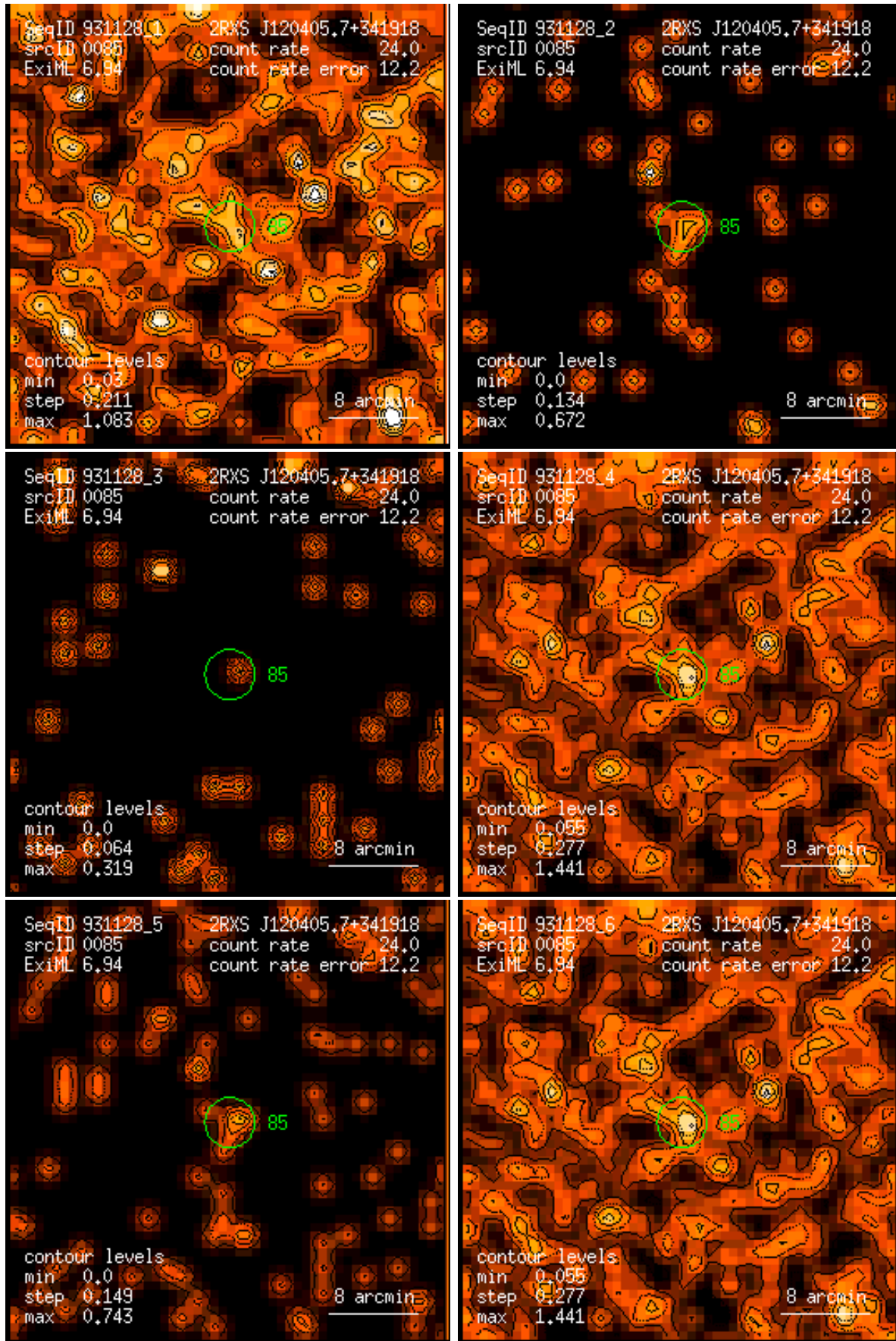
Figure 85: RASS 931128: detection 0085: band rate images, Gaussian filter: (1) PSPC channels 11 – 41, (2) 52 – 90, (3) 91 – 201, (4) 11 – 235, (5) 52 – 201, (6) 11 – 201. Broad band rates in counts/ks. Band rate contour levels in counts/ks/arcmin 2 .
