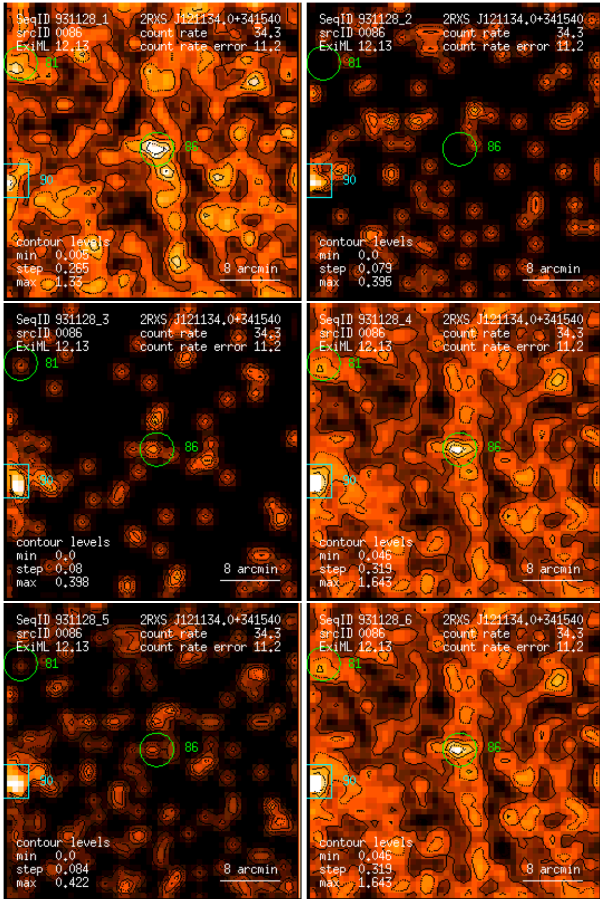
Figure 86: RASS 931128: detection 0086: band rate images, Gaussian filter: (1) PSPC channels 11 – 41, (2) 52 – 90, (3) 91 – 201, (4) 11 – 235, (5) 52 – 201, (6) 11 – 201. Broad band rates in counts/ks. Band rate contour levels in counts/ks/arcmin 2 .
