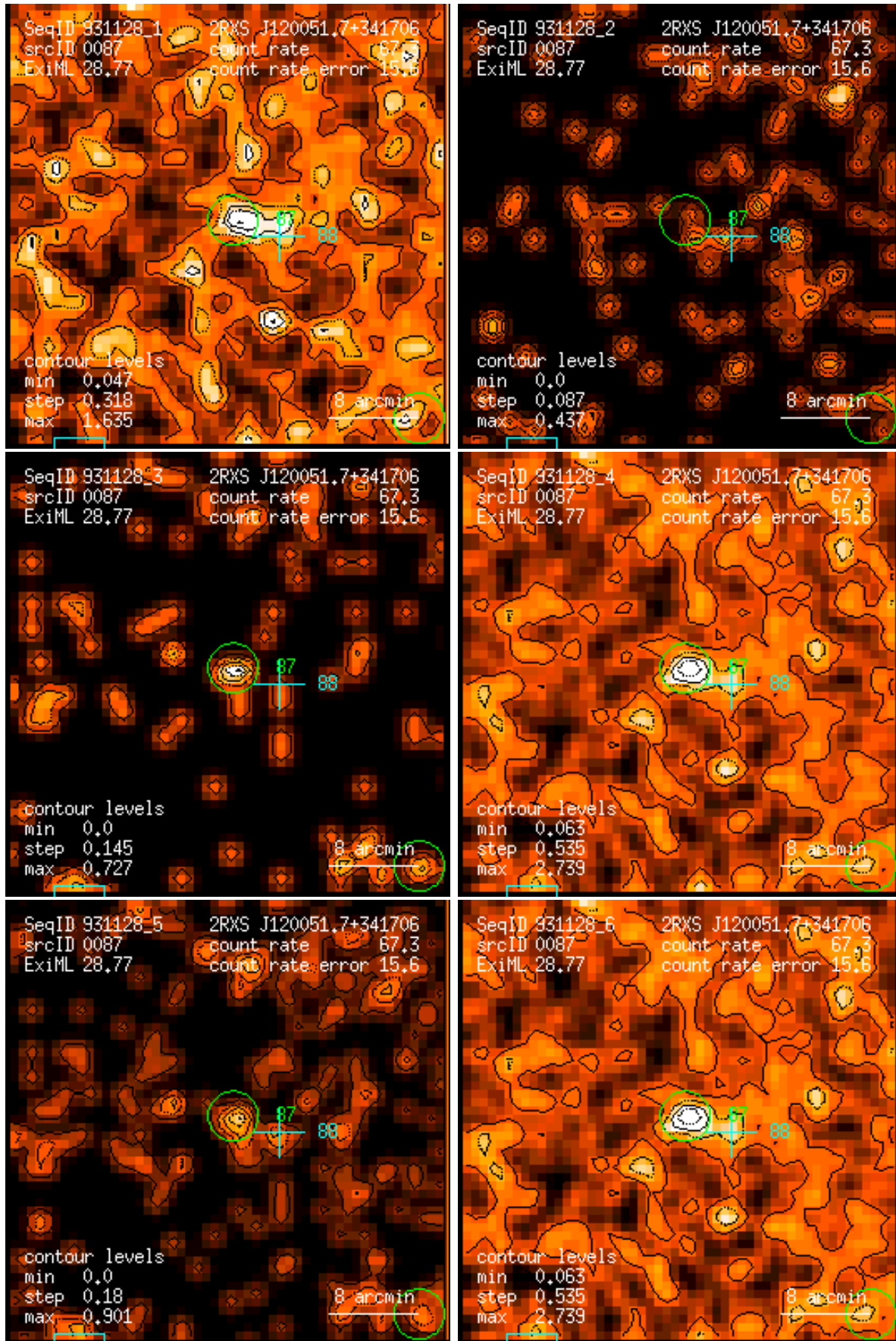
Figure 87: RASS 931128: detection 0087: band rate images, Gaussian filter: (1) PSPC channels 11 – 41, (2) 52 – 90, (3) 91 – 201, (4) 11 – 235, (5) 52 – 201, (6) 11 – 201. Broad band rates in counts/ks. Band rate contour levels in counts/ks/arcmin 2 .
