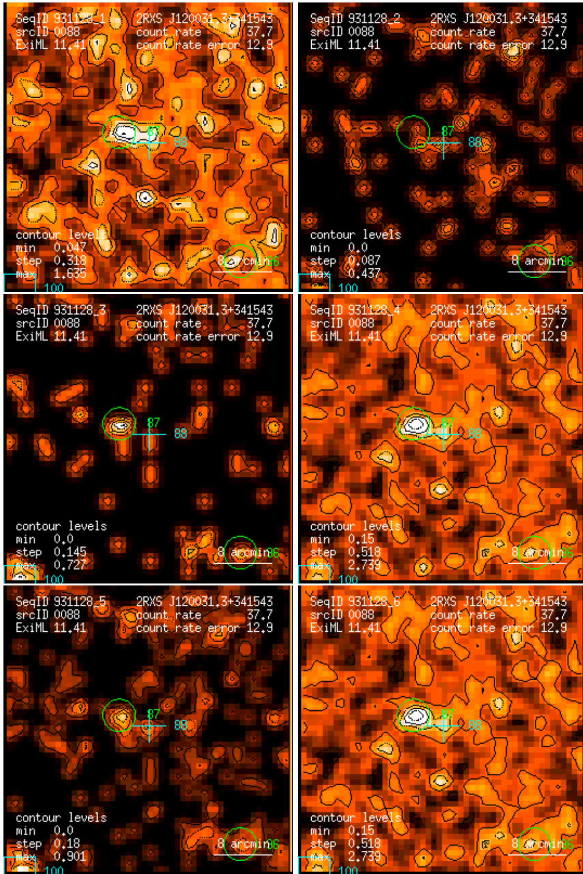
Figure 88: RASS 931128: detection 0088: band rate images, Gaussian filter: (1) PSPC channels 11 – 41, (2) 52 – 90, (3) 91 – 201, (4) 11 – 235, (5) 52 – 201, (6) 11 – 201. Broad band rates in counts/ks. Band rate contour levels in counts/ks/arcmin 2 .
