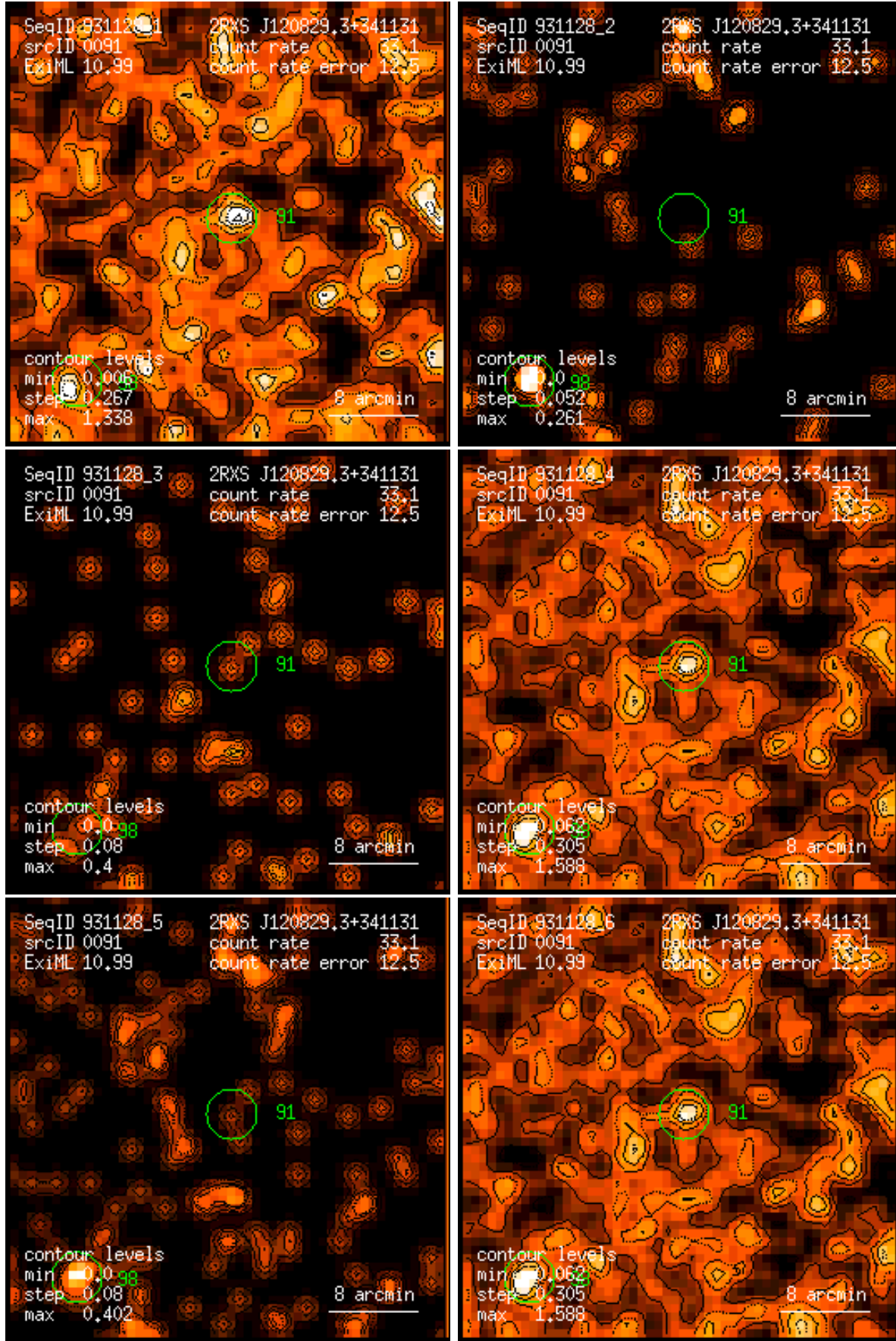
Figure 91: RASS 931128: detection 0091: band rate images, Gaussian filter: (1) PSPC channels 11 – 41, (2) 52 – 90, (3) 91 – 201, (4) 11 – 235, (5) 52 – 201, (6) 11 – 201. Broad band rates in counts/ks. Band rate contour levels in counts/ks/arcmin 2 .
