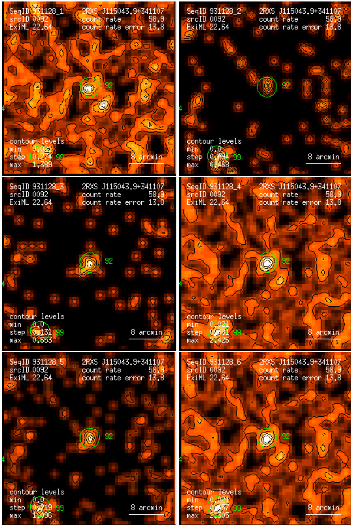
Figure 92: RASS 931128: detection 0092: band rate images, Gaussian filter: (1) PSPC channels 11 – 41, (2) 52 – 90, (3) 91 – 201, (4) 11 – 235, (5) 52 – 201, (6) 11 – 201. Broad band rates in counts/ks. Band rate contour levels in counts/ks/arcmin 2 .
